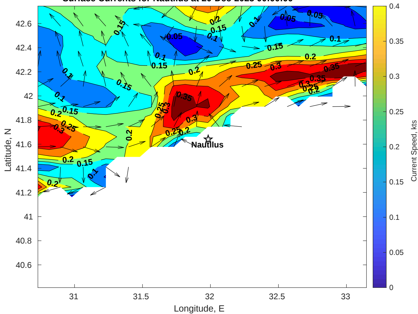
Surface Currents for Nautilus at 20-Dec-2025 00:00:00
