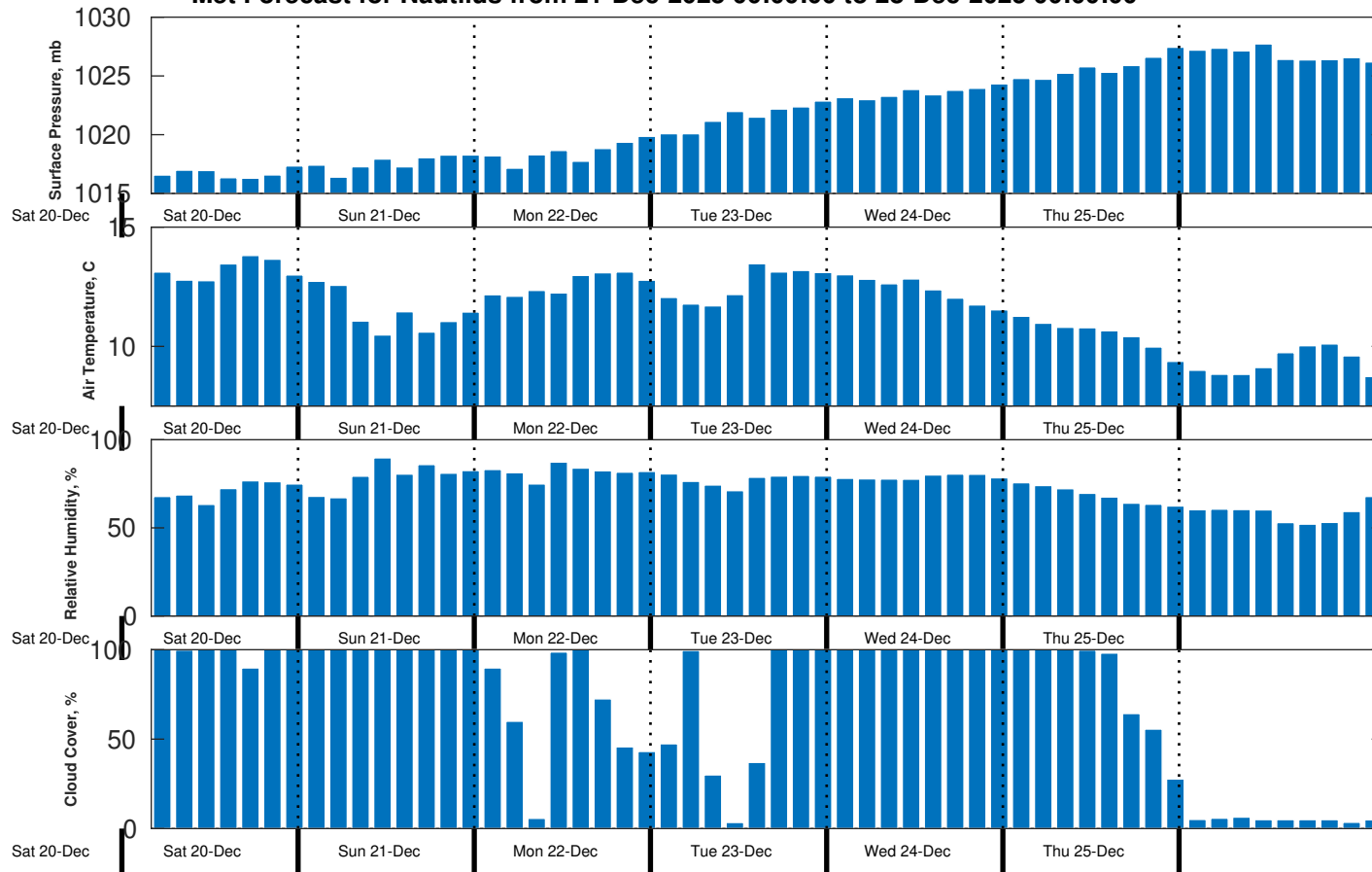
Met Forecast for Nautilus from 21-Dec-2025 00:00:00 to 28-Dec-2025 00:00:00
