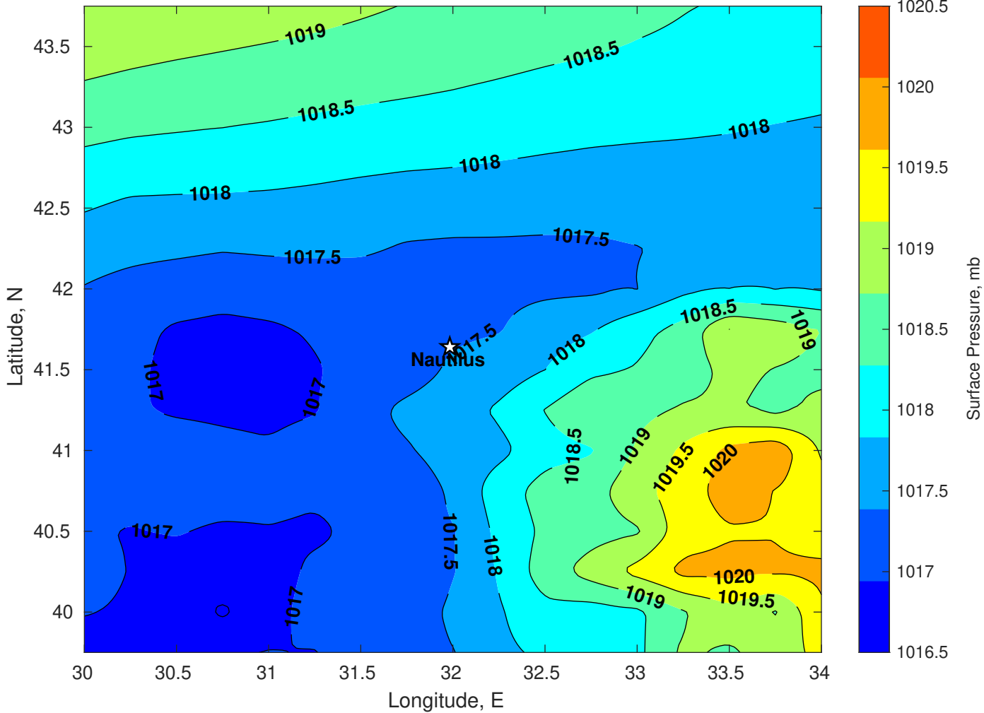
Surface Pressure (mb) for Nautilus at 22-Dec-2025 00:00:00
