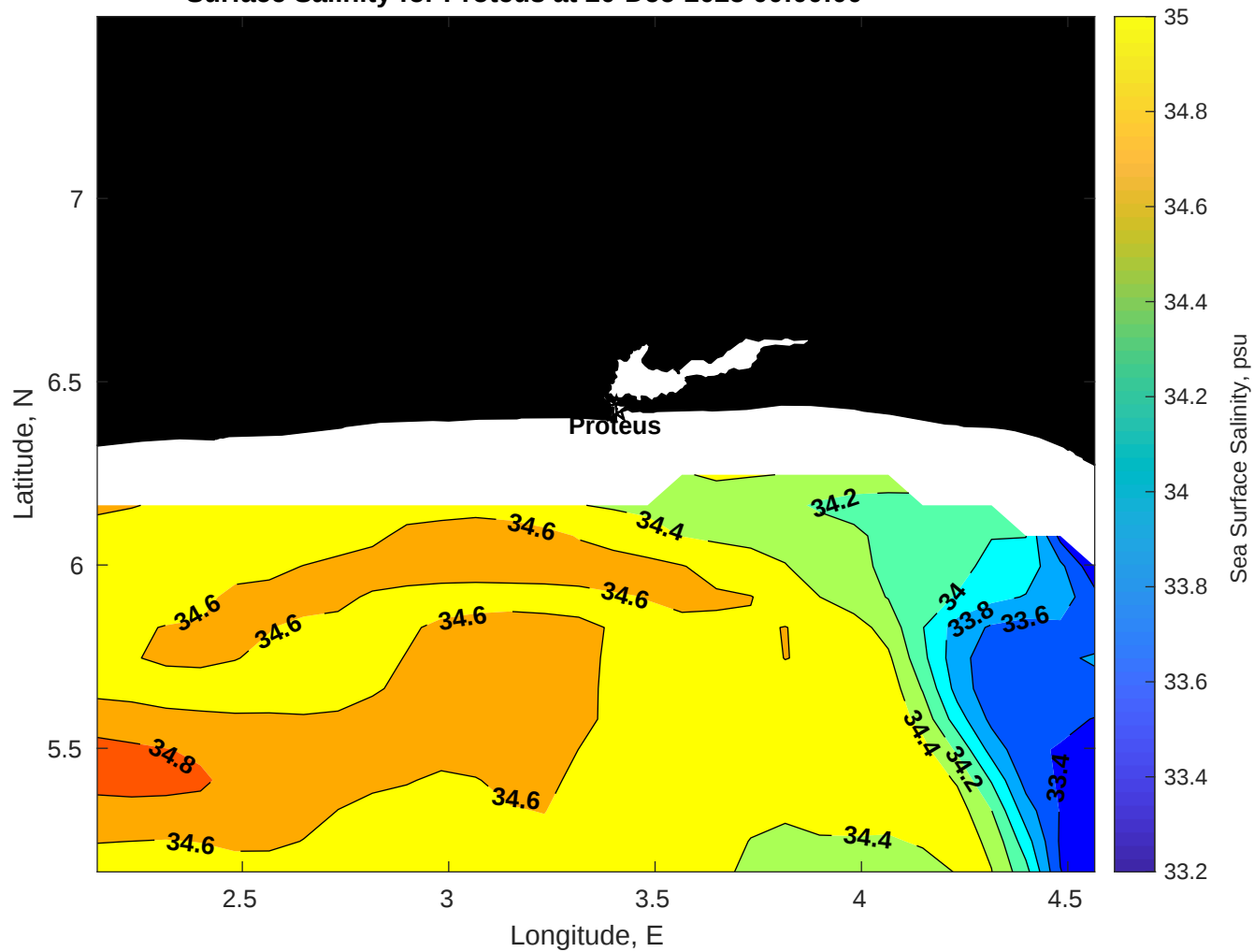
Surface Salinity for Proteus at 20-Dec-2025 00:00:00
