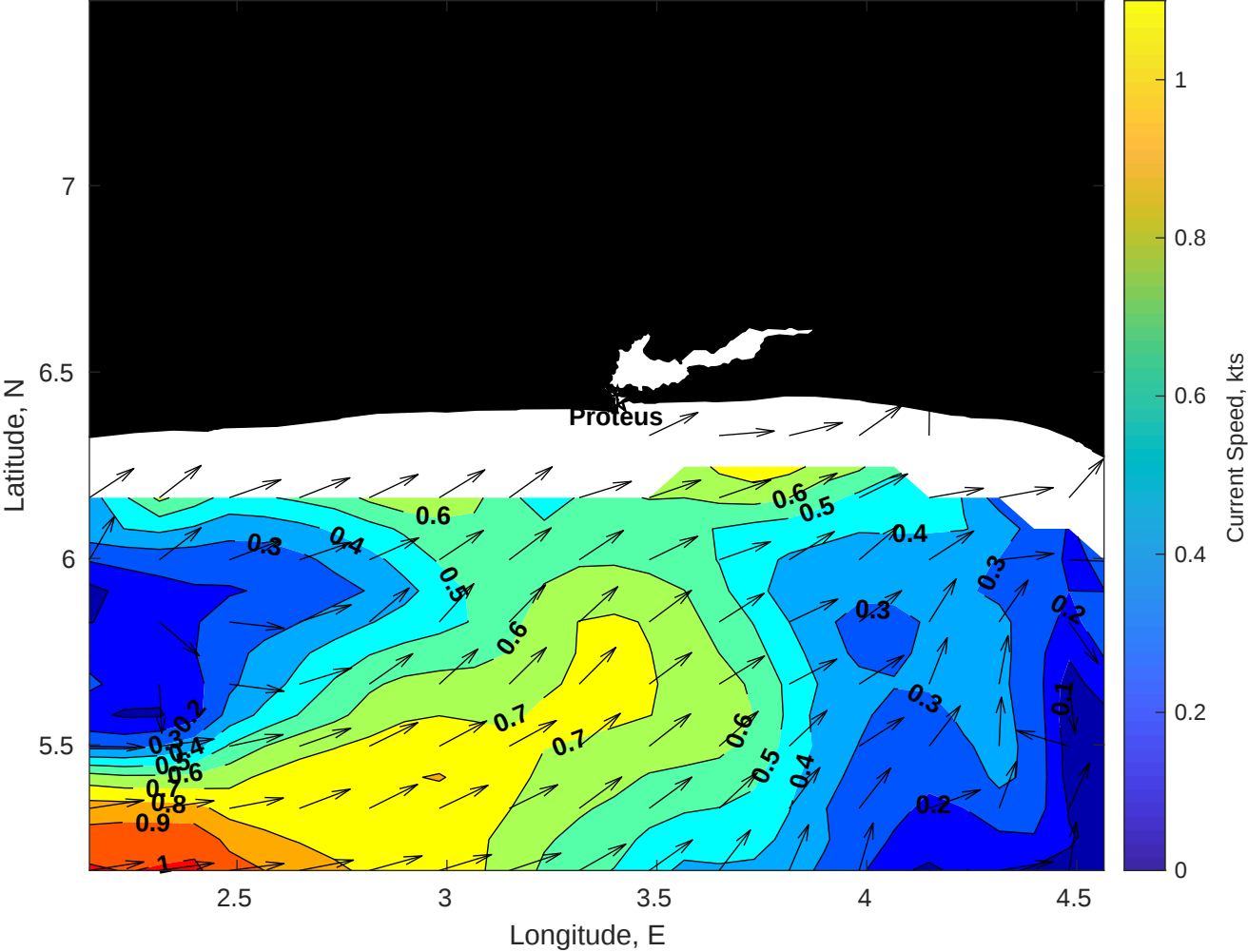
Surface Currents for Proteus at 20-Dec-2025 00:00:00
