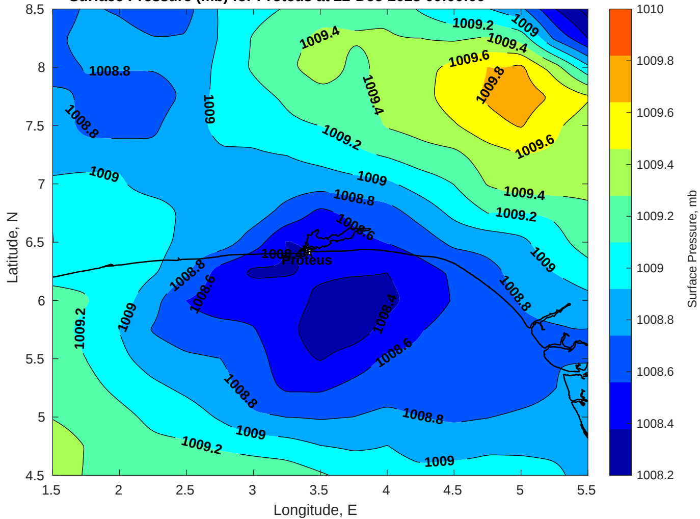
Surface Pressure (mb) for Proteus at 22-Dec-2025 00:00:00
