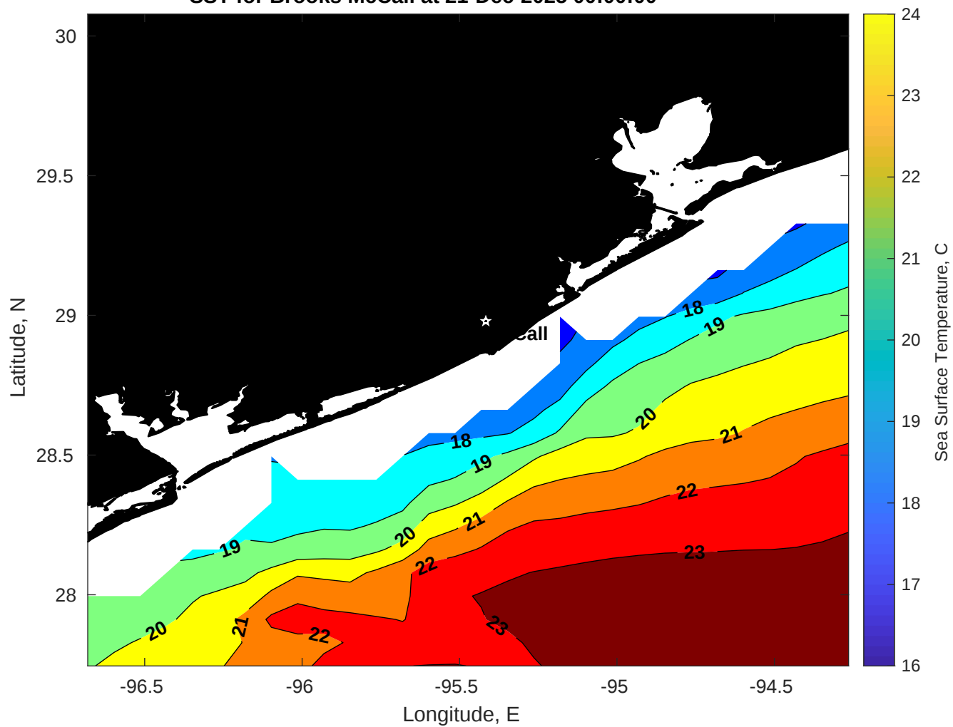
SST for Brooks McCall at 21-Dec-2025 00:00:00
