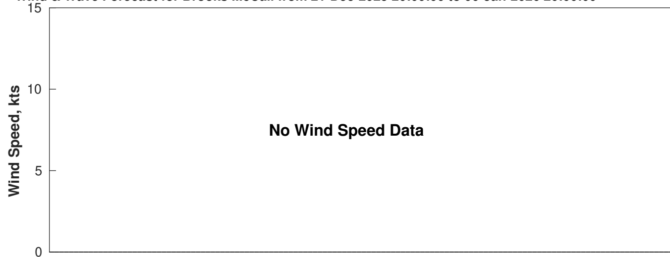
Wind & Wave Forecast for Brooks McCall from 21-Dec-2025 20:00:00 to 06-Jan-2026 20:00:00
