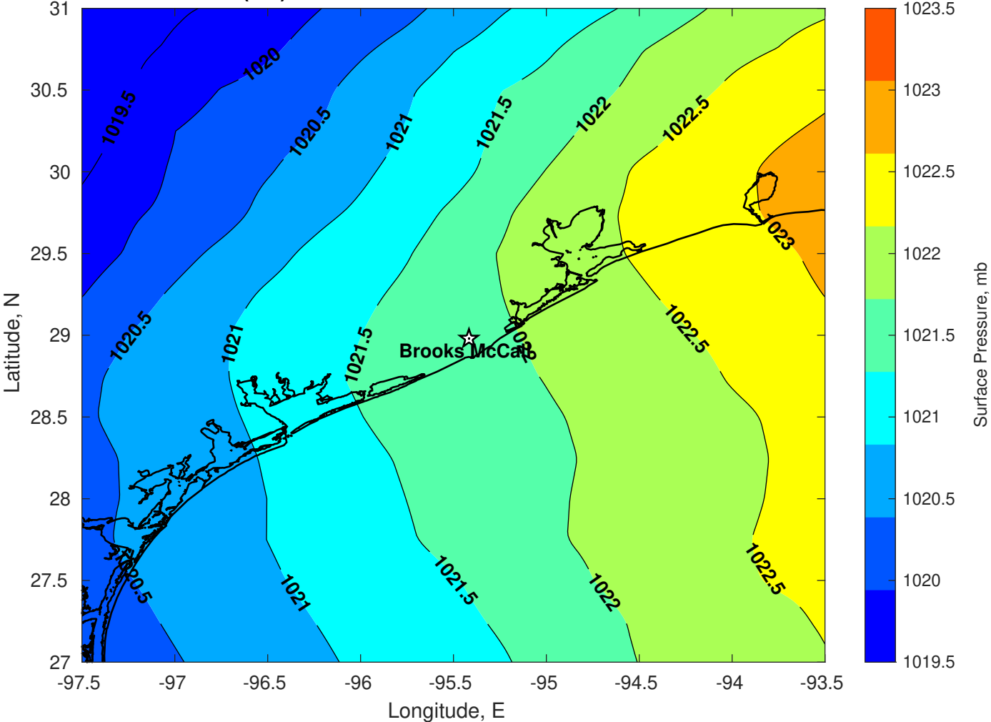
Surface Pressure (mb) for Brooks McCall at 23-Dec-2025 00:00:00
