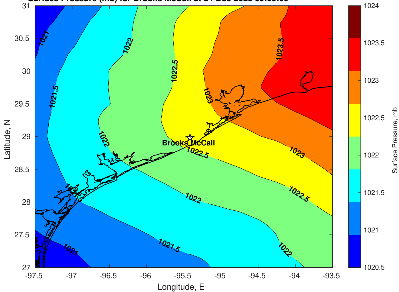
Surface Pressure (mb) for Brooks McCall at 24-Dec-2025 00:00:00
