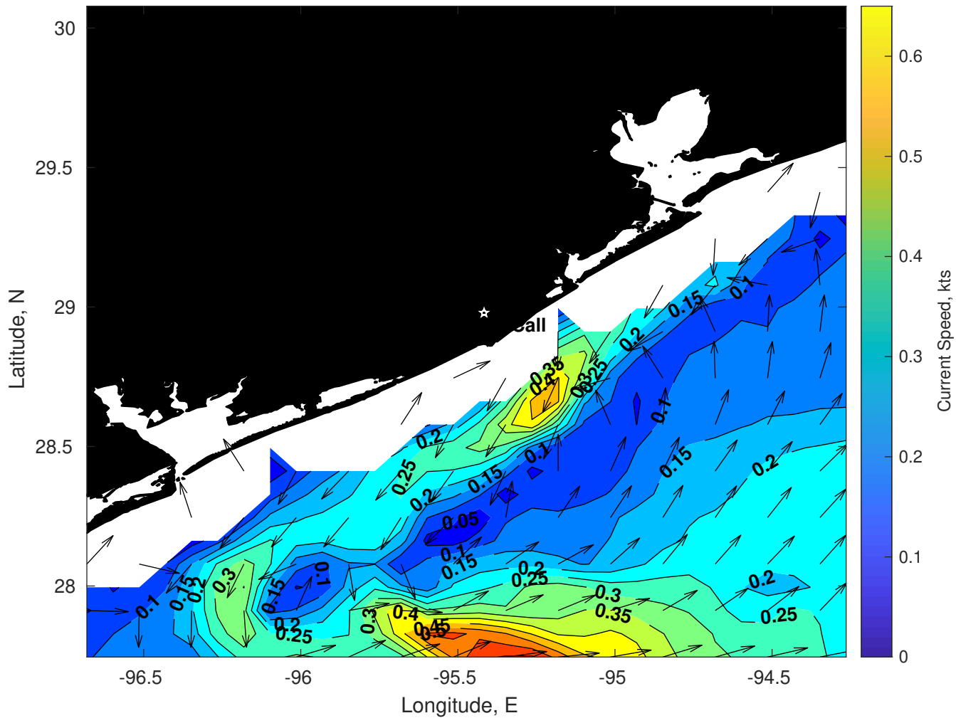
Surface Currents for Brooks McCall at 21-Dec-2025 00:00:00
