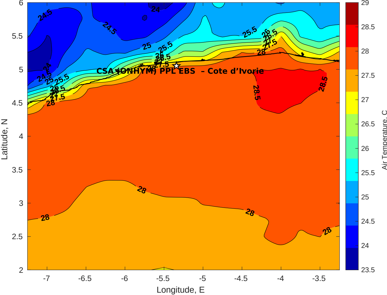
Air Temperature (C) for CSA (ONHYM) PPL EBS - Cote d'Ivoire at 22-Dec-2025
