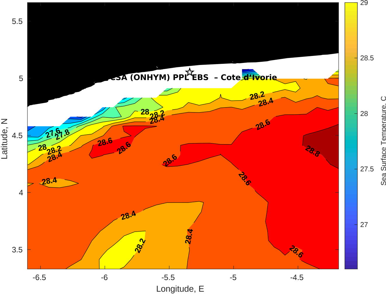
SST for CSA (ONHYM) PPL EBS - Cote d'Ivoire at 21-Dec-2025 00:00:00
