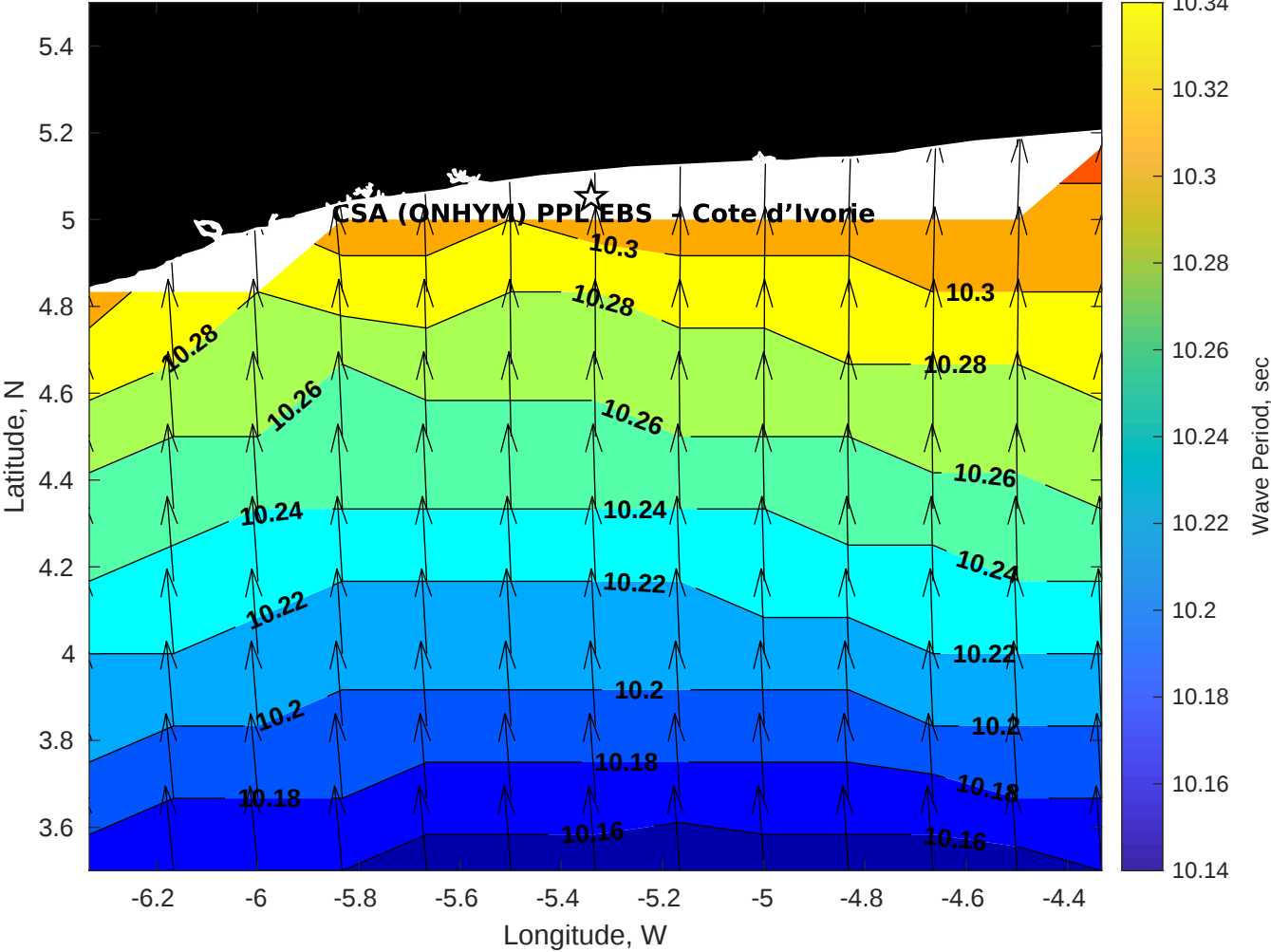
GFS Wave Period (sec) for CSA (ONHYM) PPL EBS - Cote d'Ivoire at 22-Dec-2025 09:00:00
