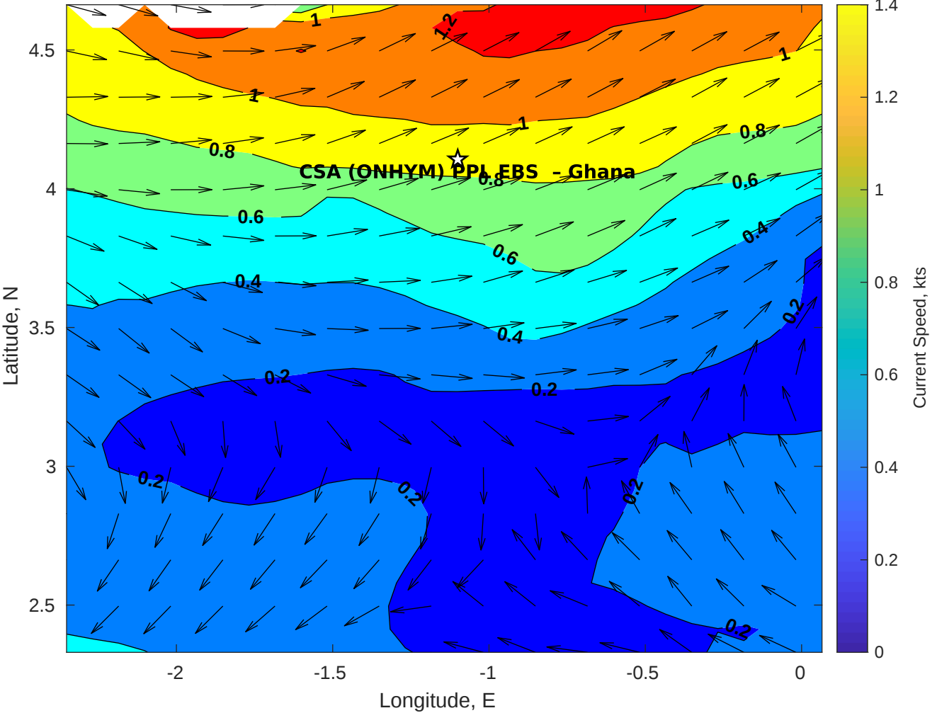
Surface Currents for CSA (ONHYM) PPL EBS - Ghana at 21-Dec-2025 00:00:00
