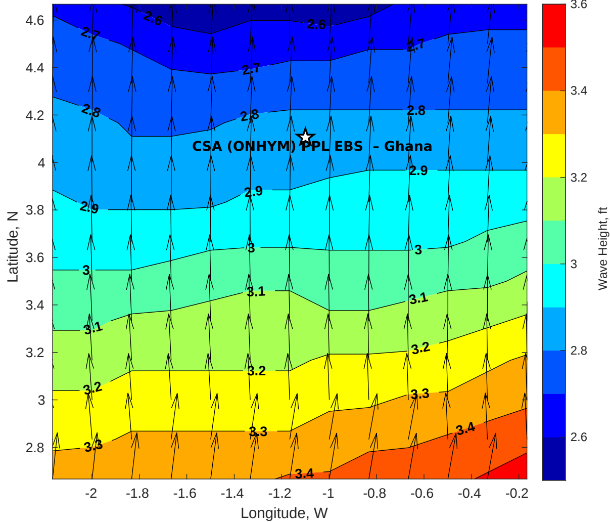
GFS Wave Height (ft) for CSA (ONHYM) PPL EBS - Ghana at 22-Dec-2025 09:00:00
