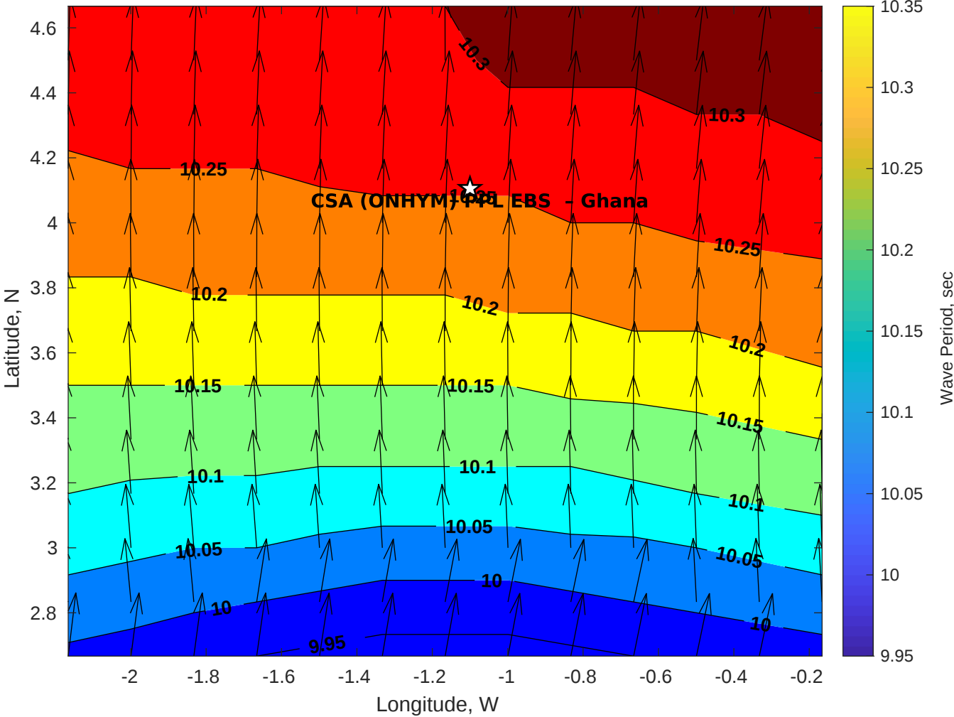
GFS Wave Period (sec) for CSA (ONHYM) PPL EBS - Ghana at 22-Dec-2025 09:00:00
