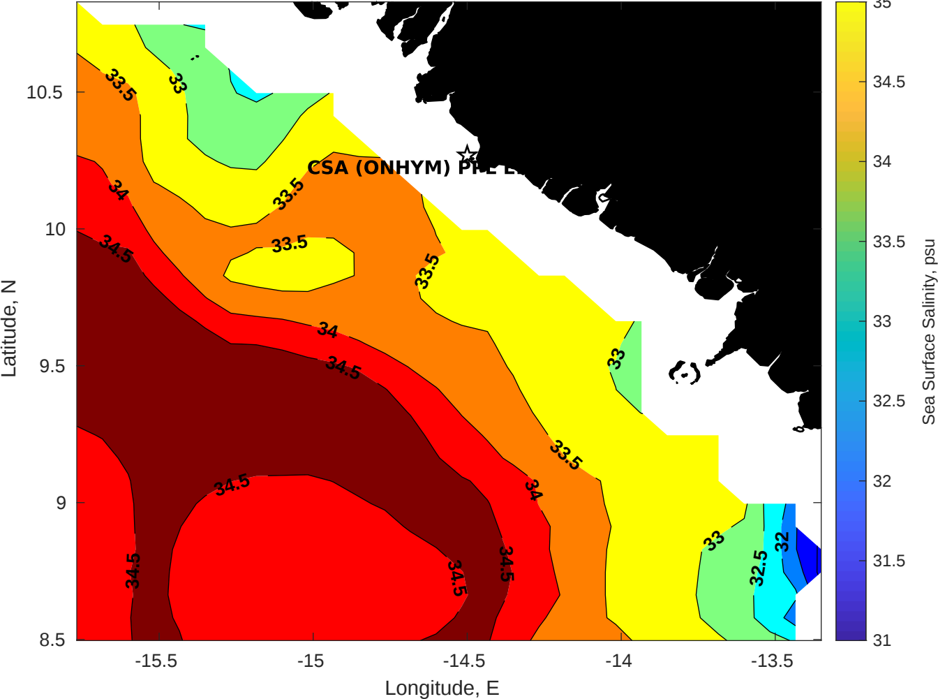
Surface Salinity for CSA (ONHYM) PPL EBS - Guinea at 21-Dec-2025 00:00:00
