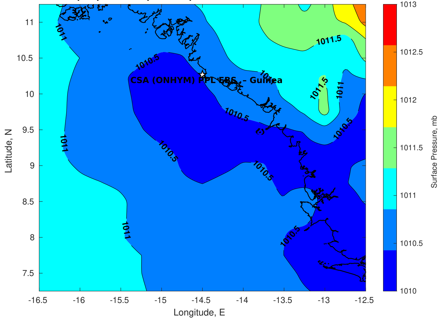
Surface Pressure (mb) for CSA (ONHYM) PPL EBS - Guinea at 22-Dec-2025 00:00:00
