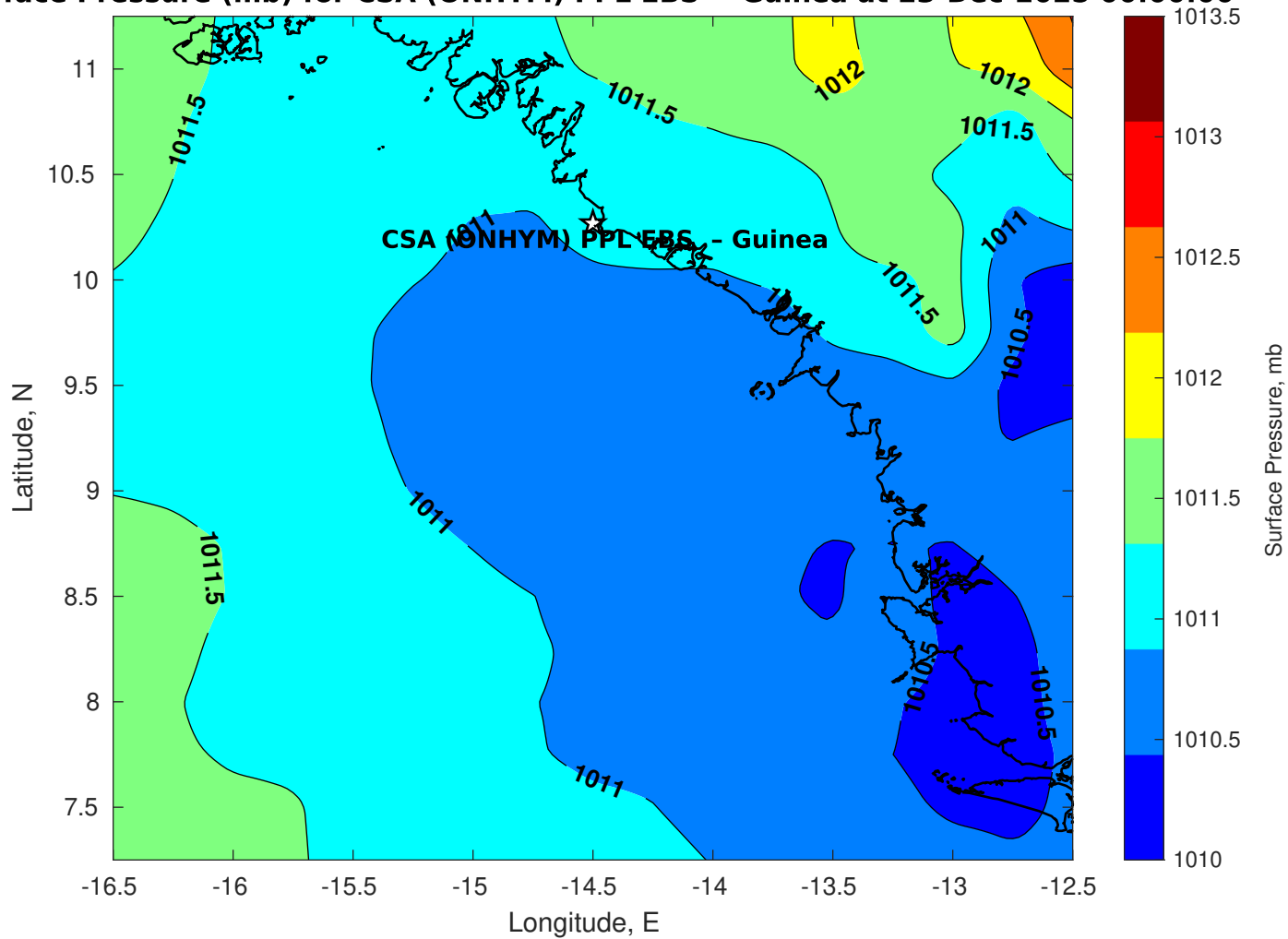
Surface Pressure (mb) for CSA (ONHYM) PPL EBS - Guinea at 23-Dec-2025 00:00:00
