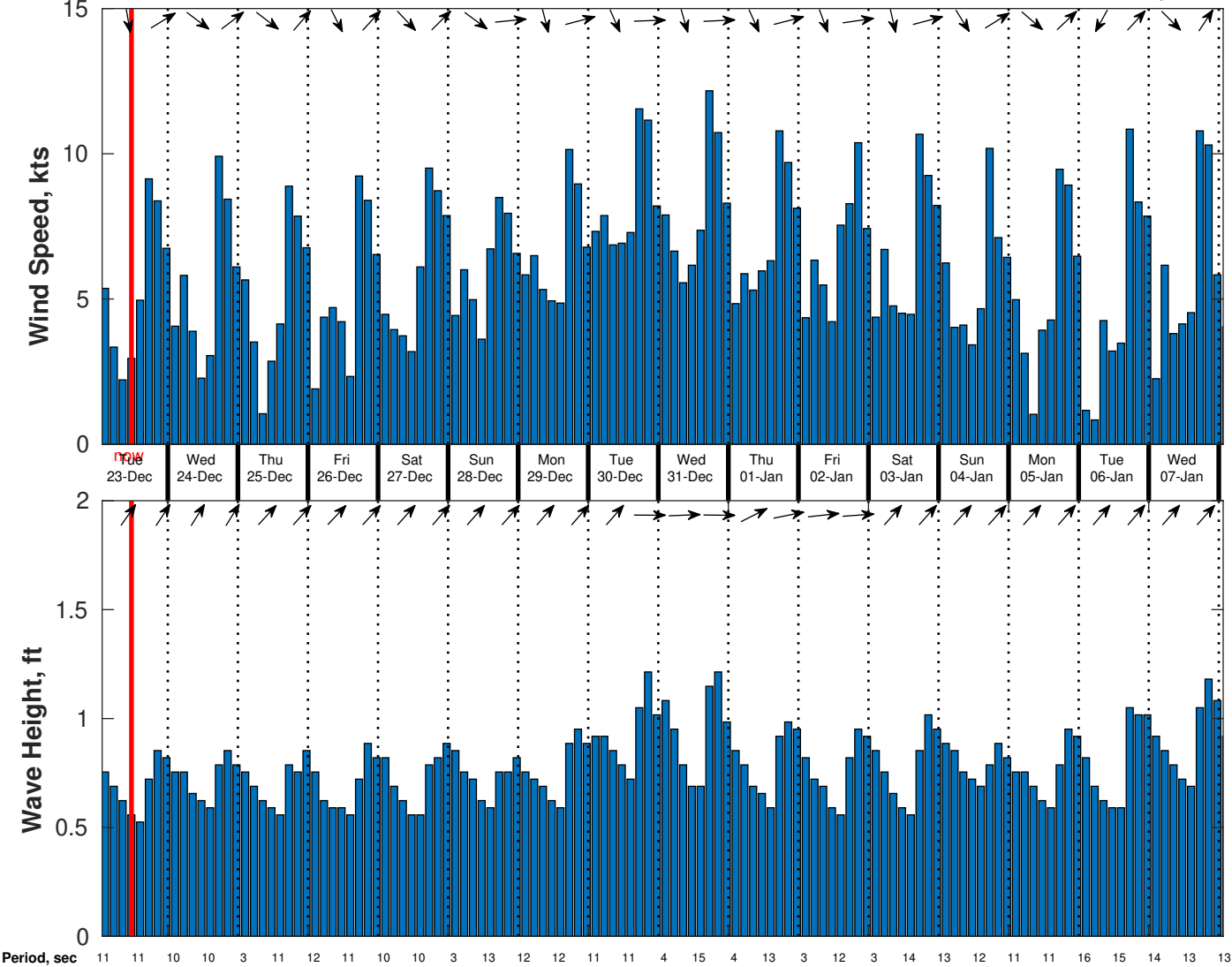
Wind & Wave Forecast for CSA (ONHYM) PPL EBS - Guinea from 22-Dec-2025 01:00:00 to 07-Jan-2026 01:00:00
