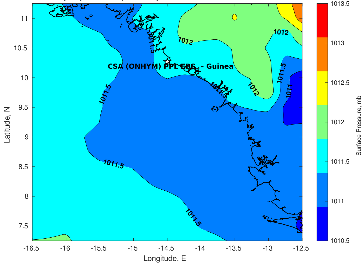
Surface Pressure (mb) for CSA (ONHYM) PPL EBS - Guinea at 24-Dec-2025 00:00:00
