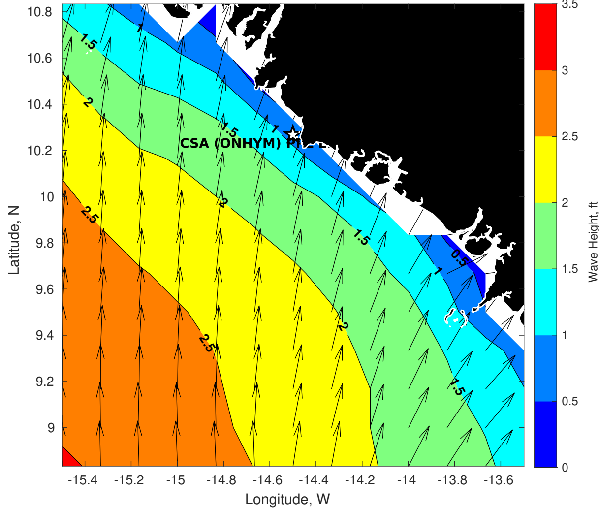
GFS Wave Height (ft) for CSA (ONHYM) PPL EBS - Guinea at 22-Dec-2025 09:00:00
