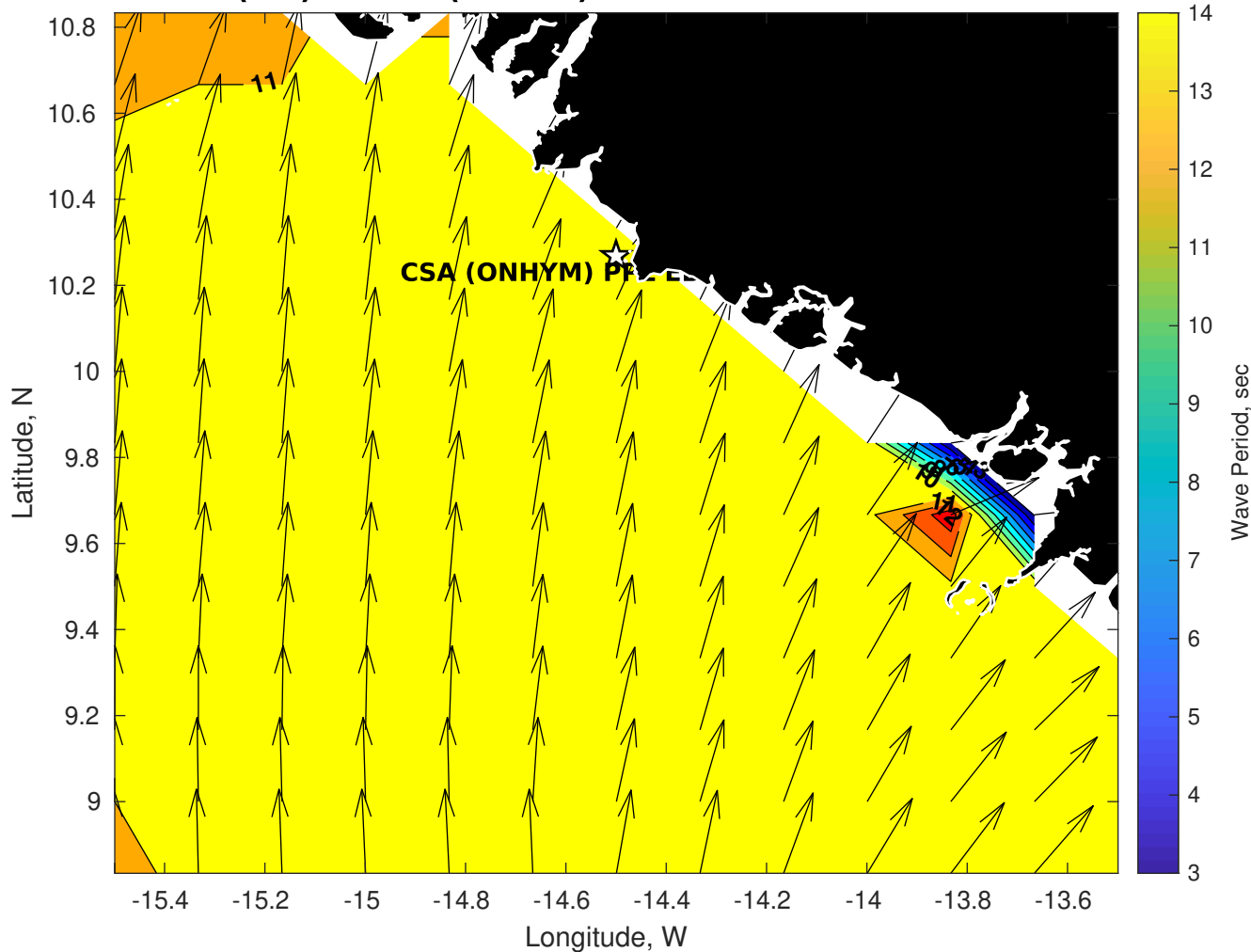
GFS Wave Period (sec) for CSA (ONHYM) PPL EBS - Guinea at 22-Dec-2025 09:00:00
