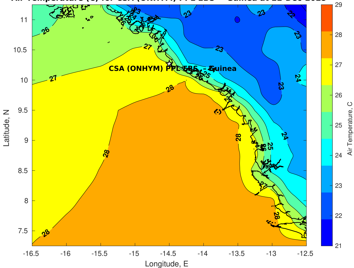
Air Temperature (C) for CSA (ONHYM) PPL EBS - Guinea at 22-Dec-2025
