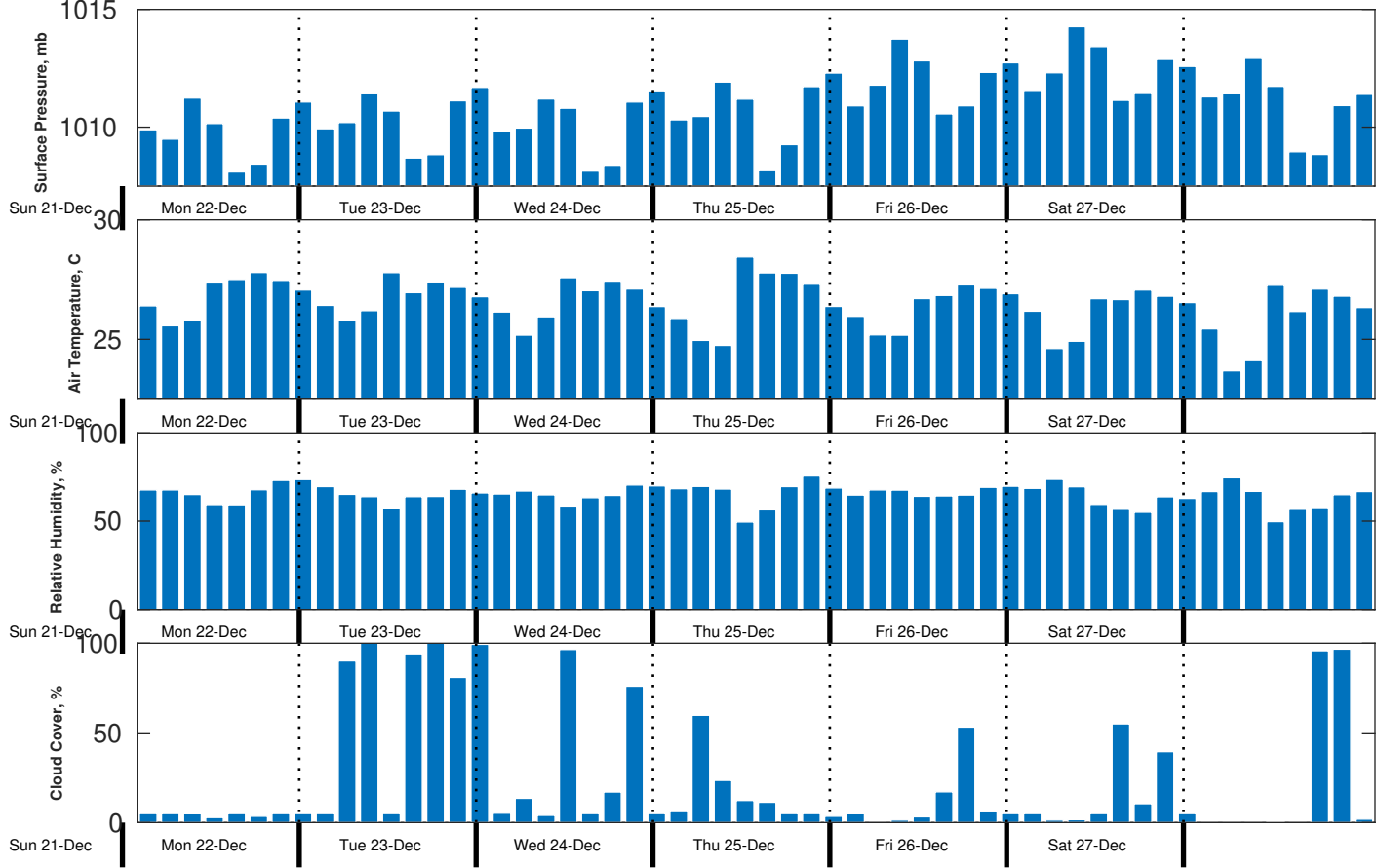
Met Forecast for CSA (ONHYM) PPL EBS - Guinea from 22-Dec-2025 00:00:00 to 29-Dec-2025 00:00:00
