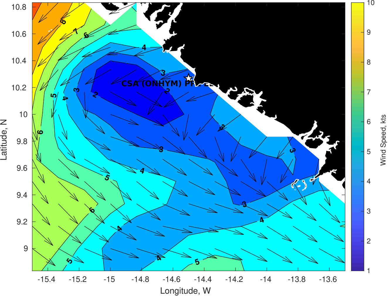
GFS Winds (kts) for CSA (ONHYM) PPL EBS - Guinea at 22-Dec-2025 09:00:00
