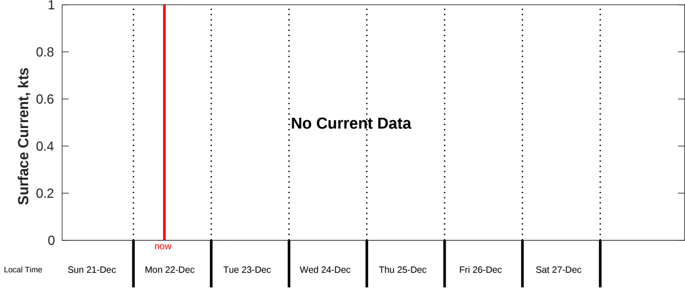
Surface Current Forecast for CSA (ONHYM) PPL EBS - Guinea from 21-Dec-2025 00:00:00 to 29-Dec-2025 00:00:00
