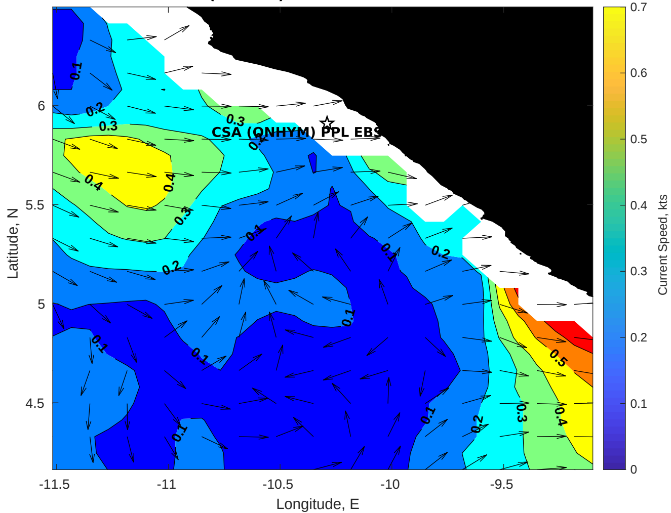
Surface Currents for CSA (ONHYM) PPL EBS - Liberia at 21-Dec-2025 00:00:00
