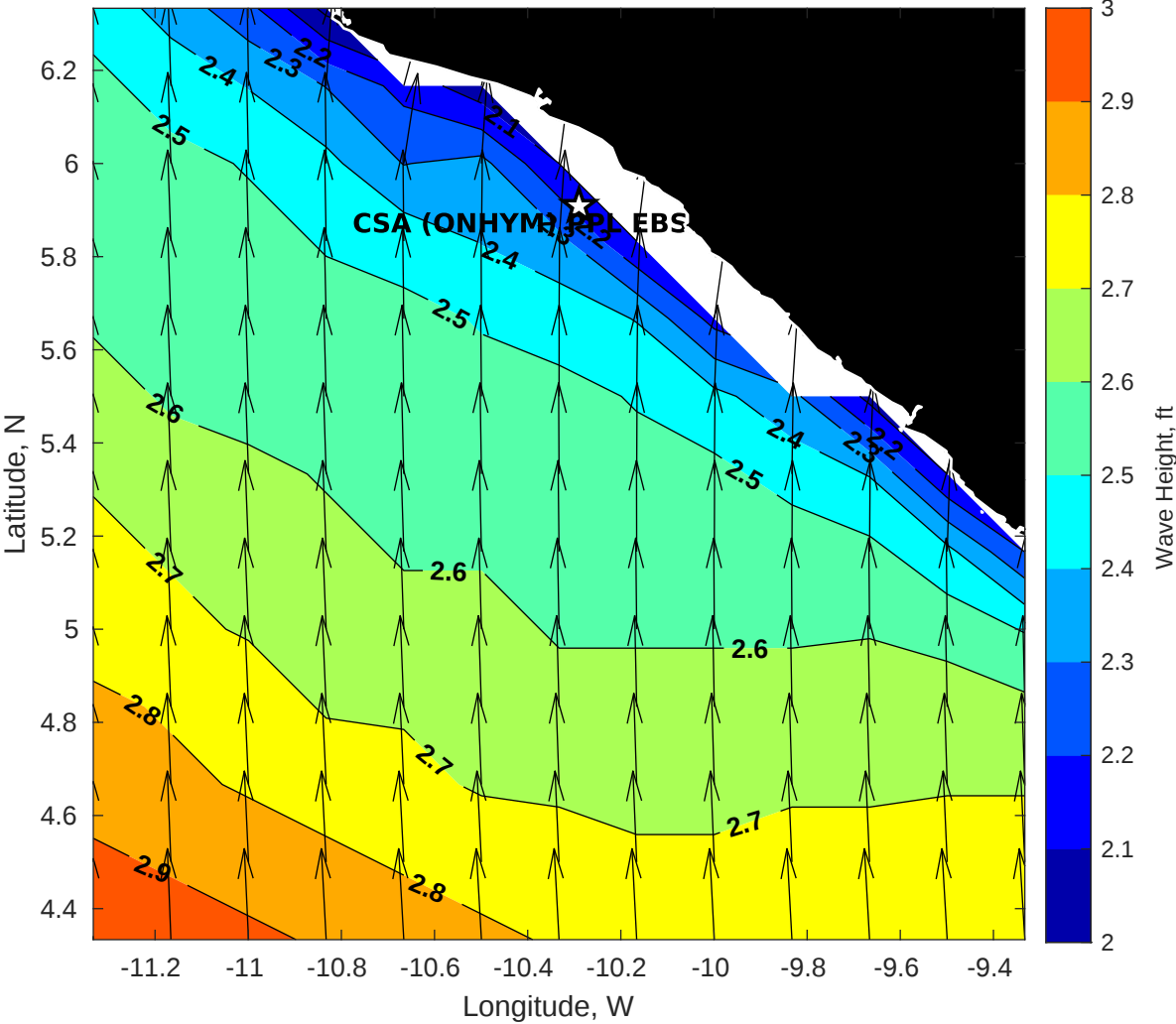
GFS Wave Height (ft) for CSA (ONHYM) PPL EBS - Liberia at 22-Dec-2025 09:00:00
