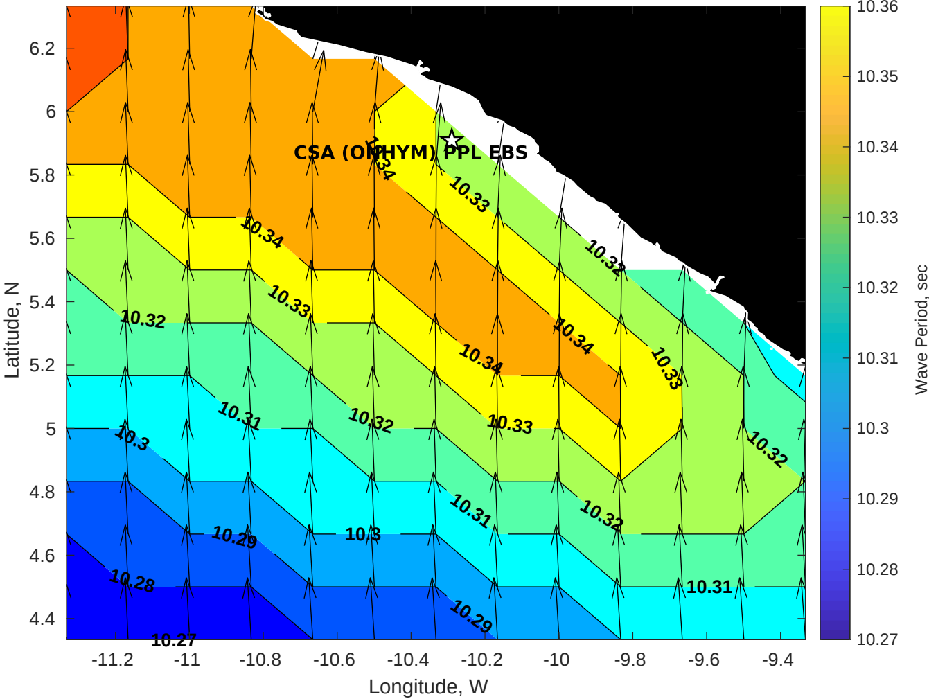
GFS Wave Period (sec) for CSA (ONHYM) PPL EBS - Liberia at 22-Dec-2025 09:00:00
