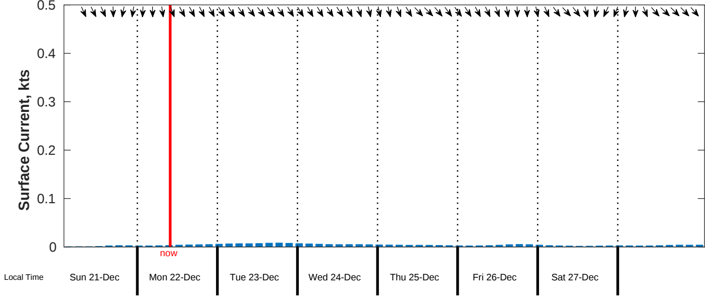
Surface Current Forecast for CSA (ONHYM) PPL EBS - Liberia from 21-Dec-2025 00:00:00 to 29-Dec-2025 00:00:00
