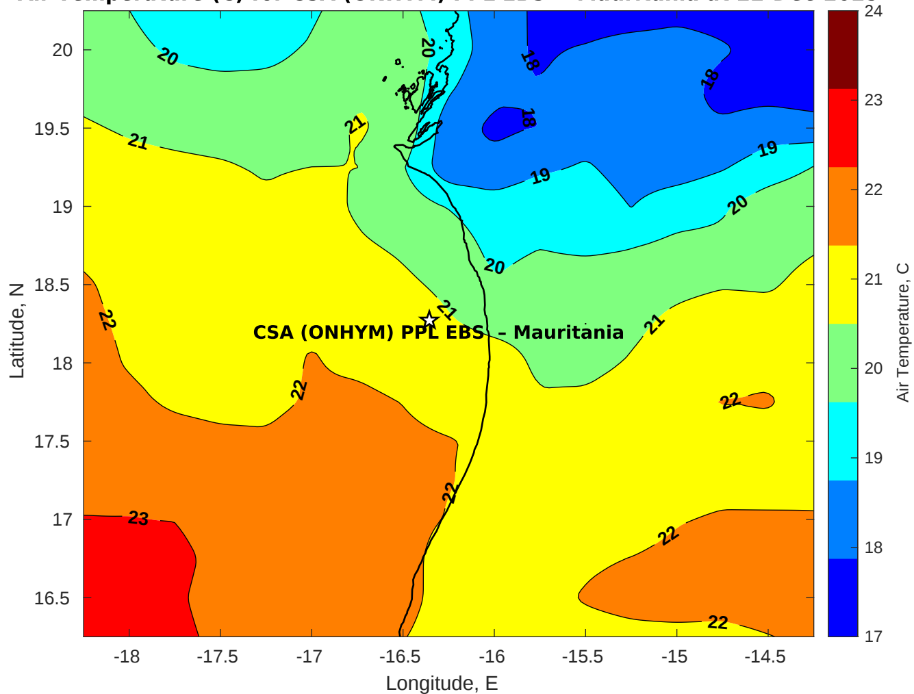
Air Temperature (C) for CSA (ONHYM) PPL EBS - Mauritania at 22-Dec-2025
