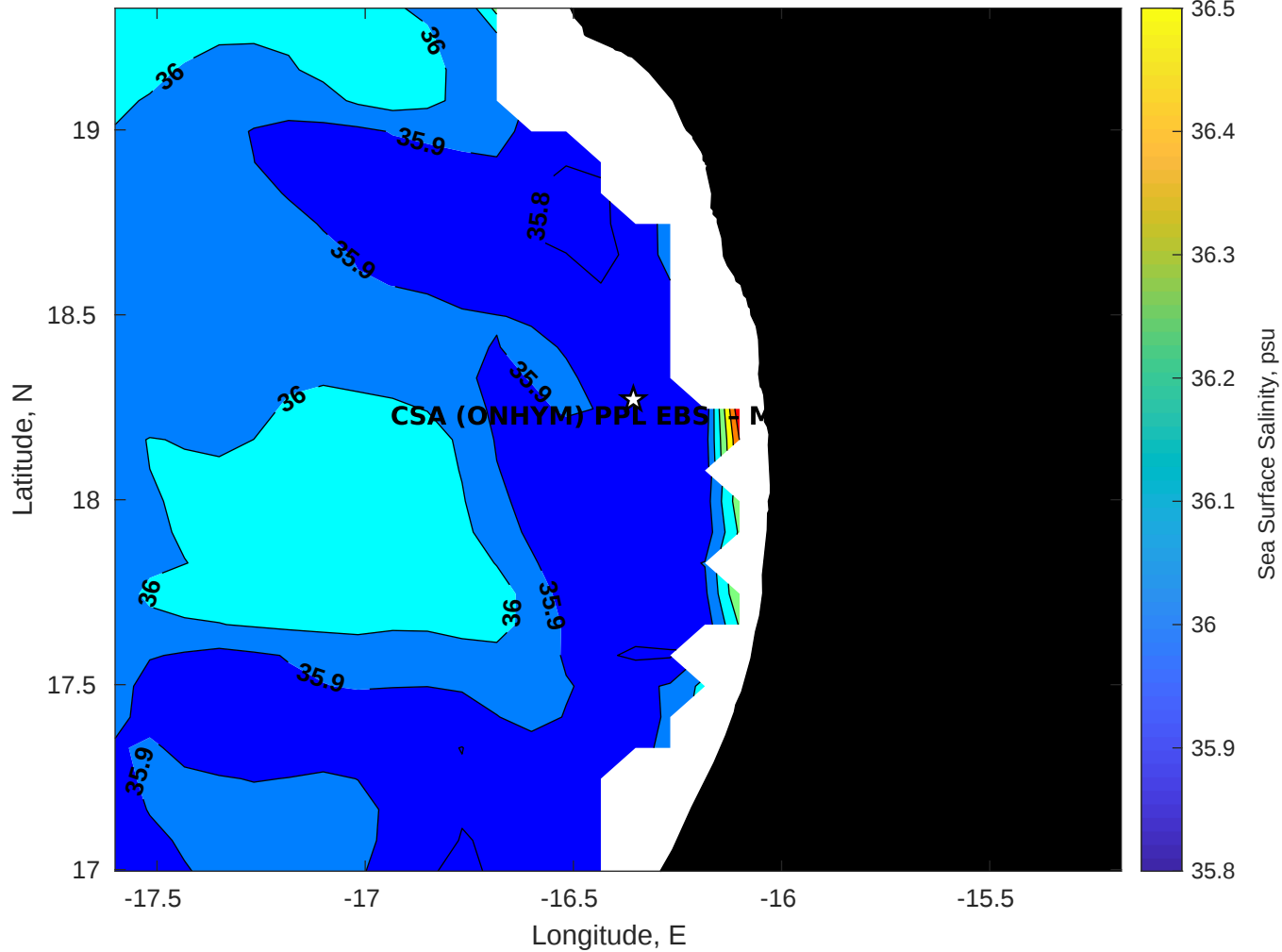
Surface Salinity for CSA (ONHYM) PPL EBS - Mauritania at 21-Dec-2025 00:00:00
