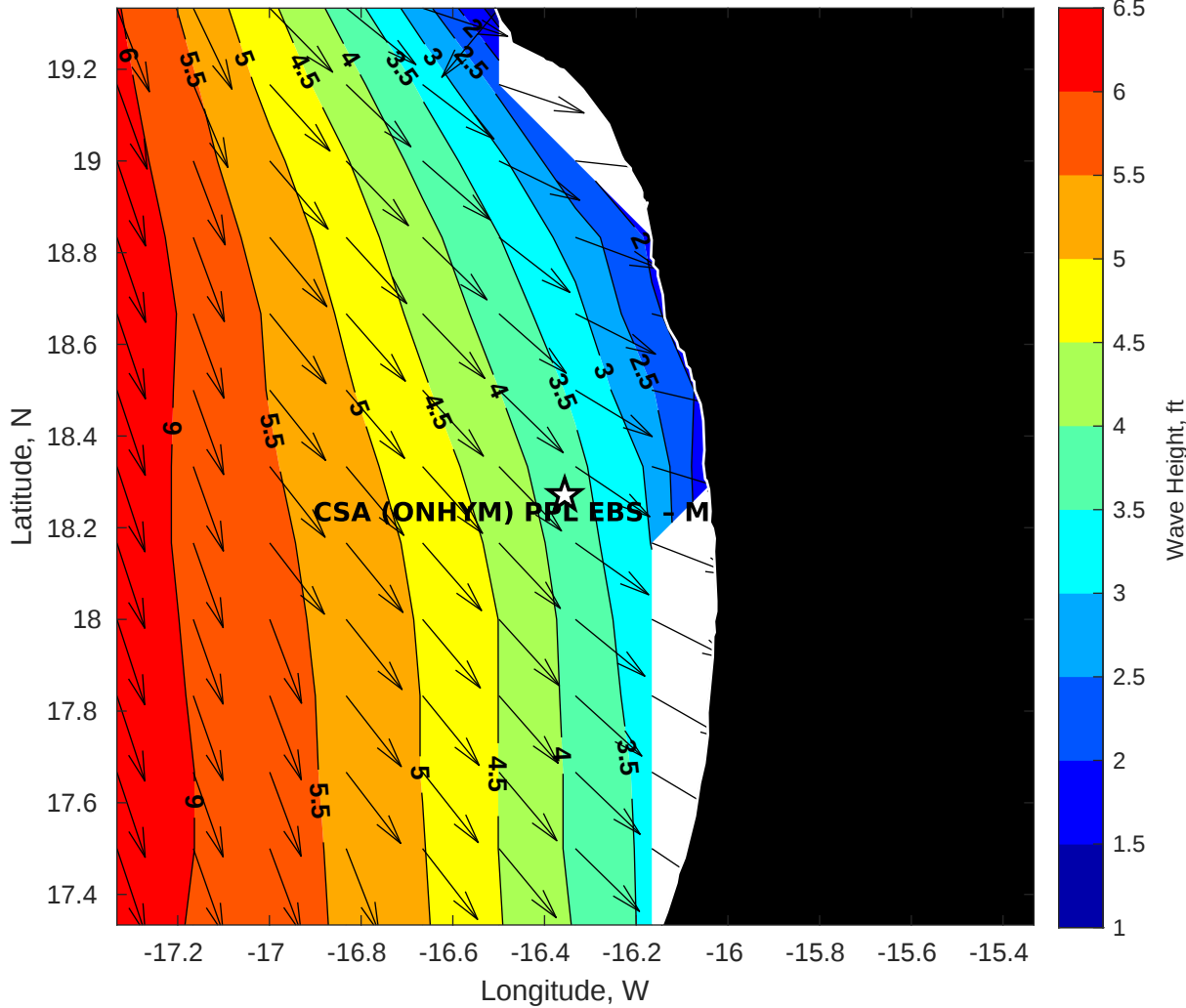
GFS Wave Height (ft) for CSA (ONHYM) PPL EBS - Mauritania at 22-Dec-2025 09:00:00
