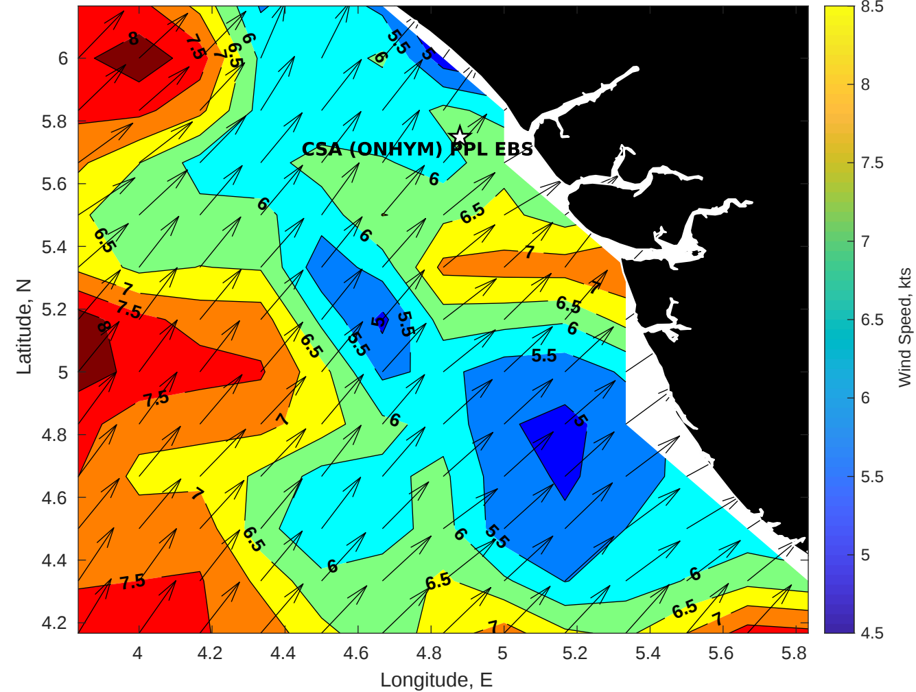
GFS Winds (kts) for CSA (ONHYM) PPL EBS - Nigeria at 22-Dec-2025 09:00:00
