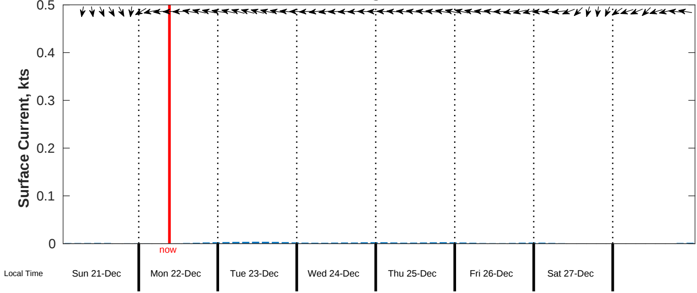
Surface Current Forecast for CSA (ONHYM) PPL EBS - Nigeria from 21-Dec-2025 00:00:00 to 29-Dec-2025 00:00:00
