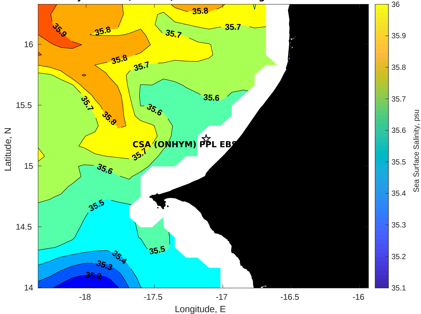
Surface Salinity for CSA (ONHYM) PPL EBS - Senegal at 21-Dec-2025 00:00:00
