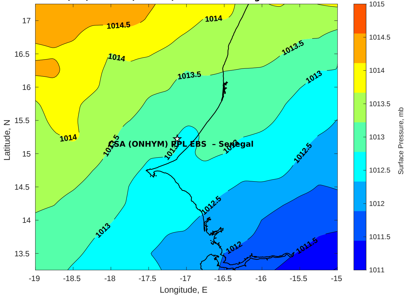
Surface Pressure (mb) for CSA (ONHYM) PPL EBS - Senegal at 23-Dec-2025 00:00:00
