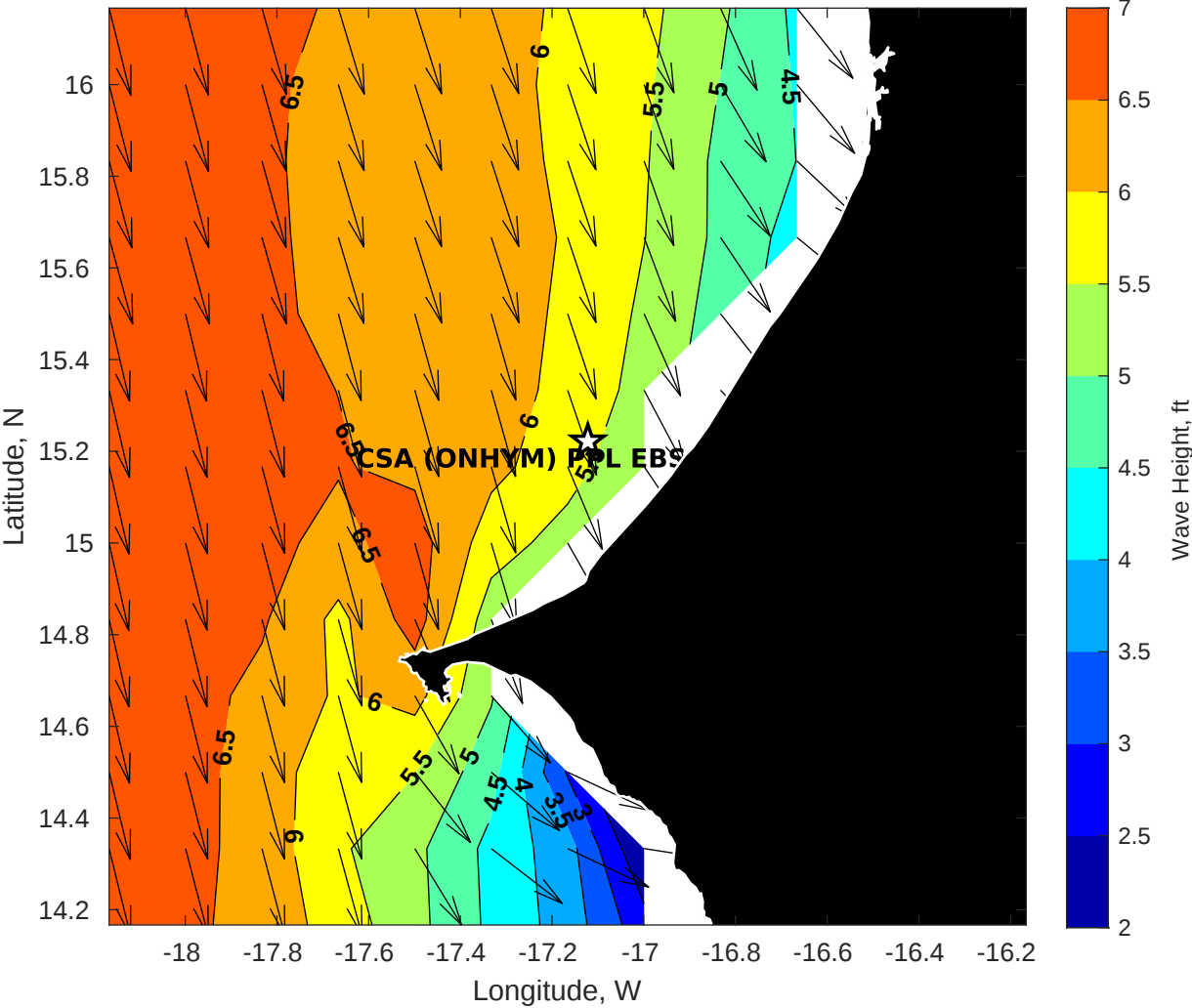
GFS Wave Height (ft) for CSA (ONHYM) PPL EBS - Senegal at 22-Dec-2025 09:00:00
