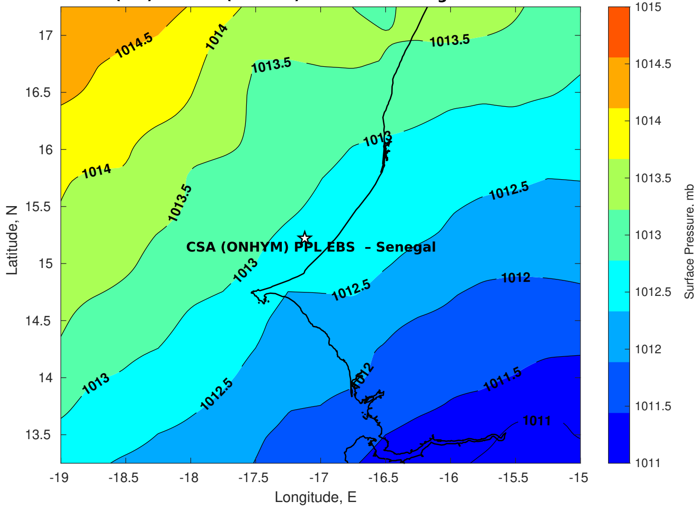
Surface Pressure (mb) for CSA (ONHYM) PPL EBS - Senegal at 22-Dec-2025 00:00:00
