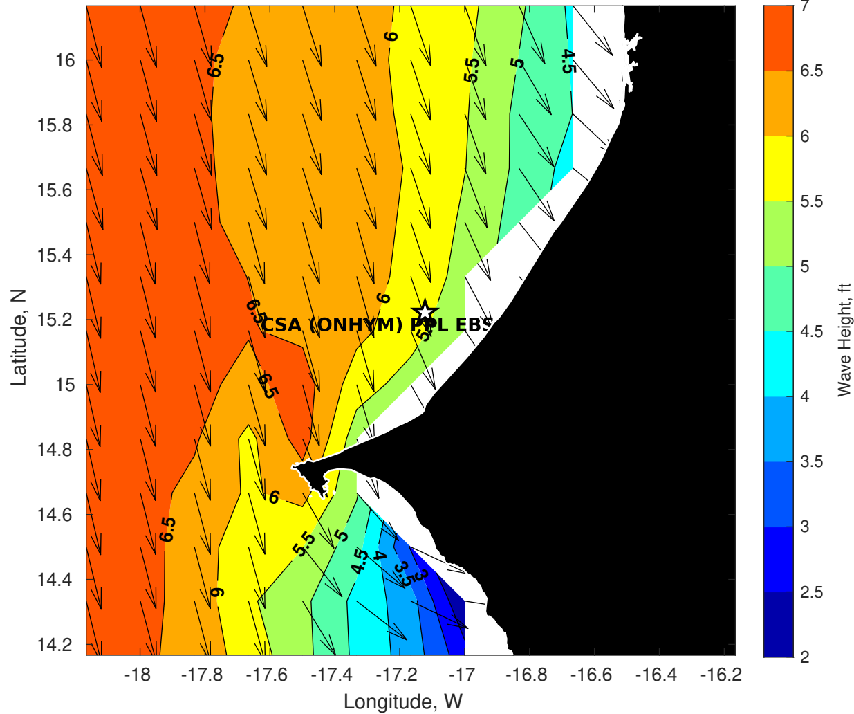
GFS Wave Height (ft) for CSA (ONHYM) PPL EBS - Senegal at 22-Dec-2025 09:00:00
