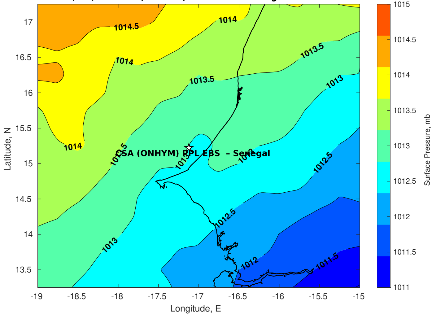
Surface Pressure (mb) for CSA (ONHYM) PPL EBS - Senegal at 23-Dec-2025 00:00:00
