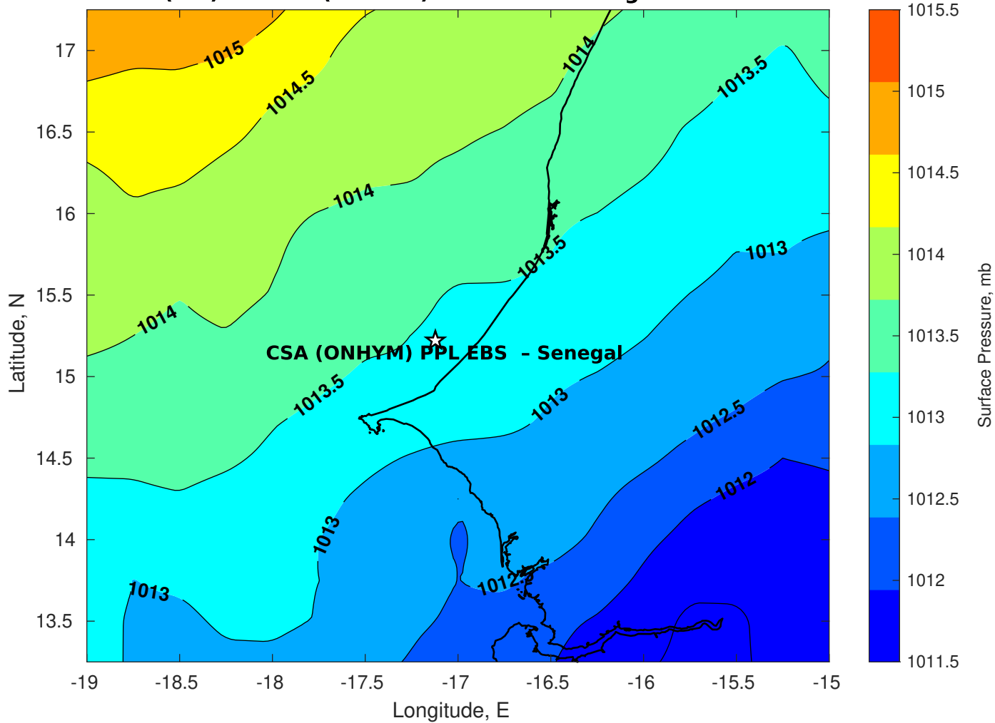
Surface Pressure (mb) for CSA (ONHYM) PPL EBS - Senegal at 24-Dec-2025 00:00:00
