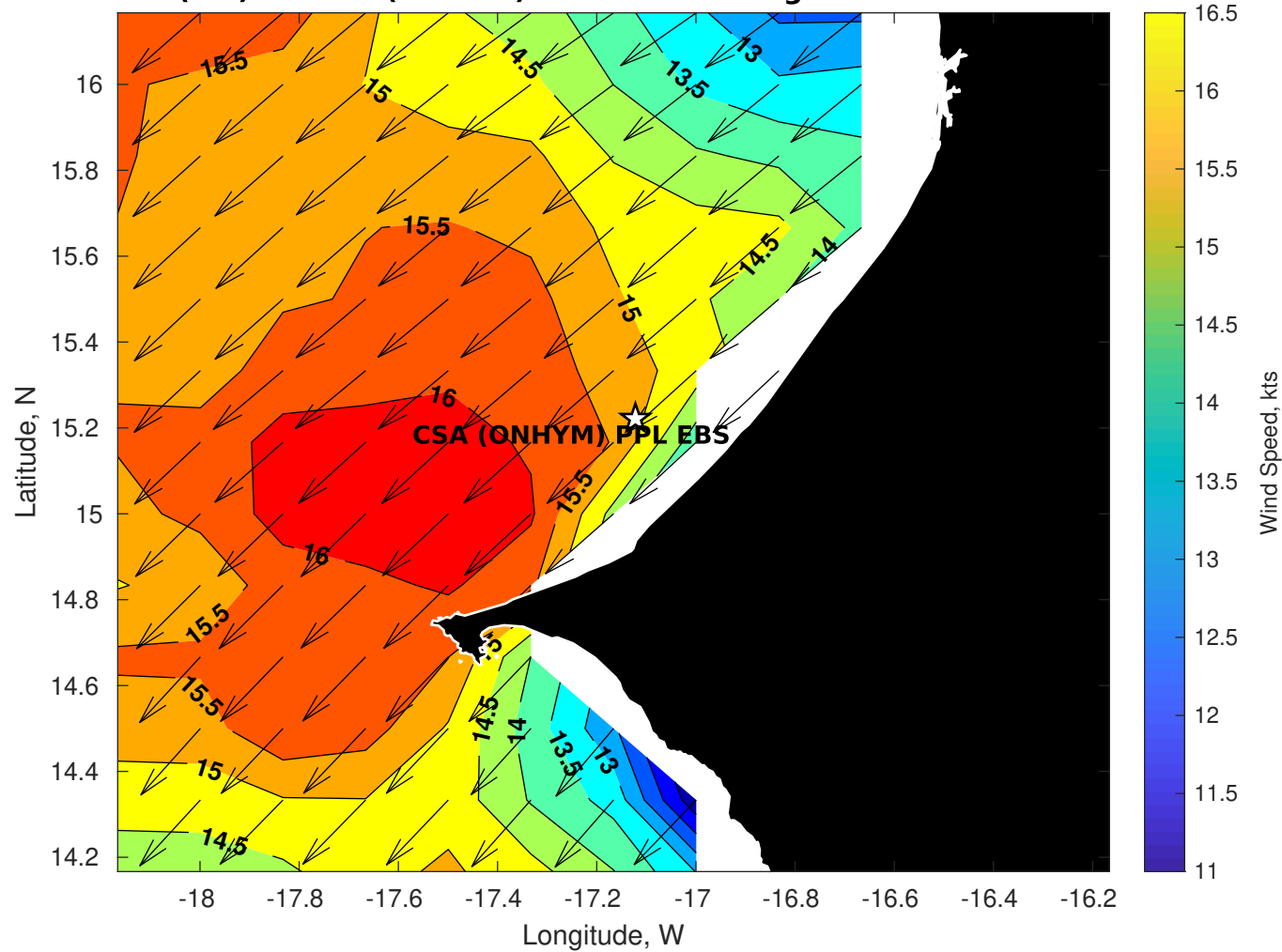
GFS Winds (kts) for CSA (ONHYM) PPL EBS - Senegal at 22-Dec-2025 09:00:00
