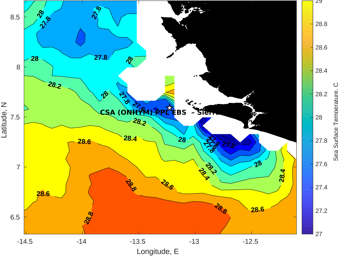
SST for CSA (ONHYM) PPL EBS - Sierra Leone at 21-Dec-2025 00:00:00
