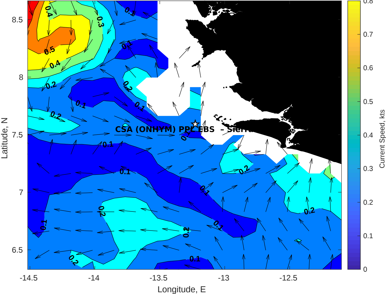
Surface Currents for CSA (ONHYM) PPL EBS - Sierra Leone at 21-Dec-2025 00:00:00
