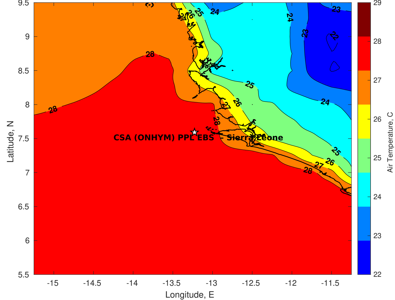
Air Temperature (C) for CSA (ONHYM) PPL EBS - Sierra Leone at 22-Dec-2025
