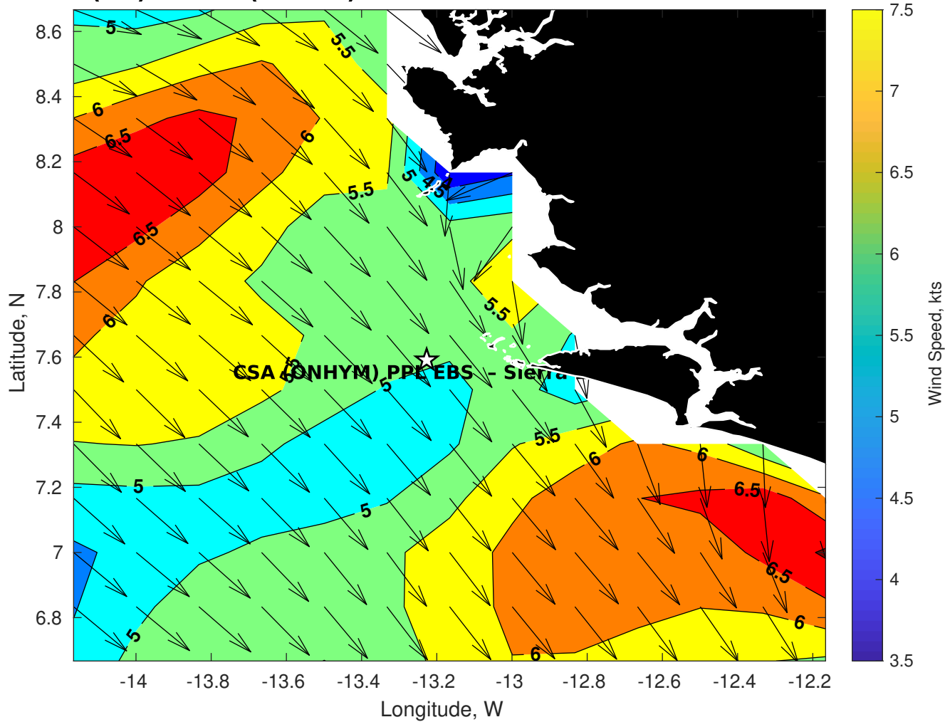
GFS Winds (kts) for CSA (ONHYM) PPL EBS - Sierra Leone at 22-Dec-2025 09:00:00
