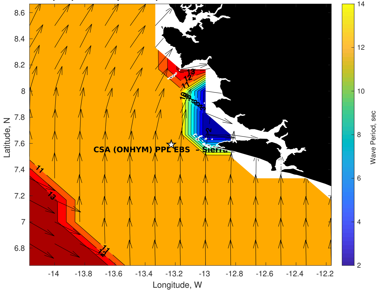
GFS Wave Period (sec) for CSA (ONHYM) PPL EBS - Sierra Leone at 22-Dec-2025 09:00:00
