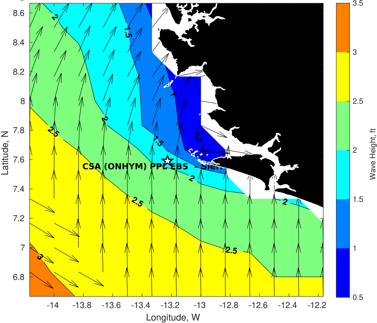
GFS Wave Height (ft) for CSA (ONHYM) PPL EBS - Sierra Leone at 22-Dec-2025 09:00:00
