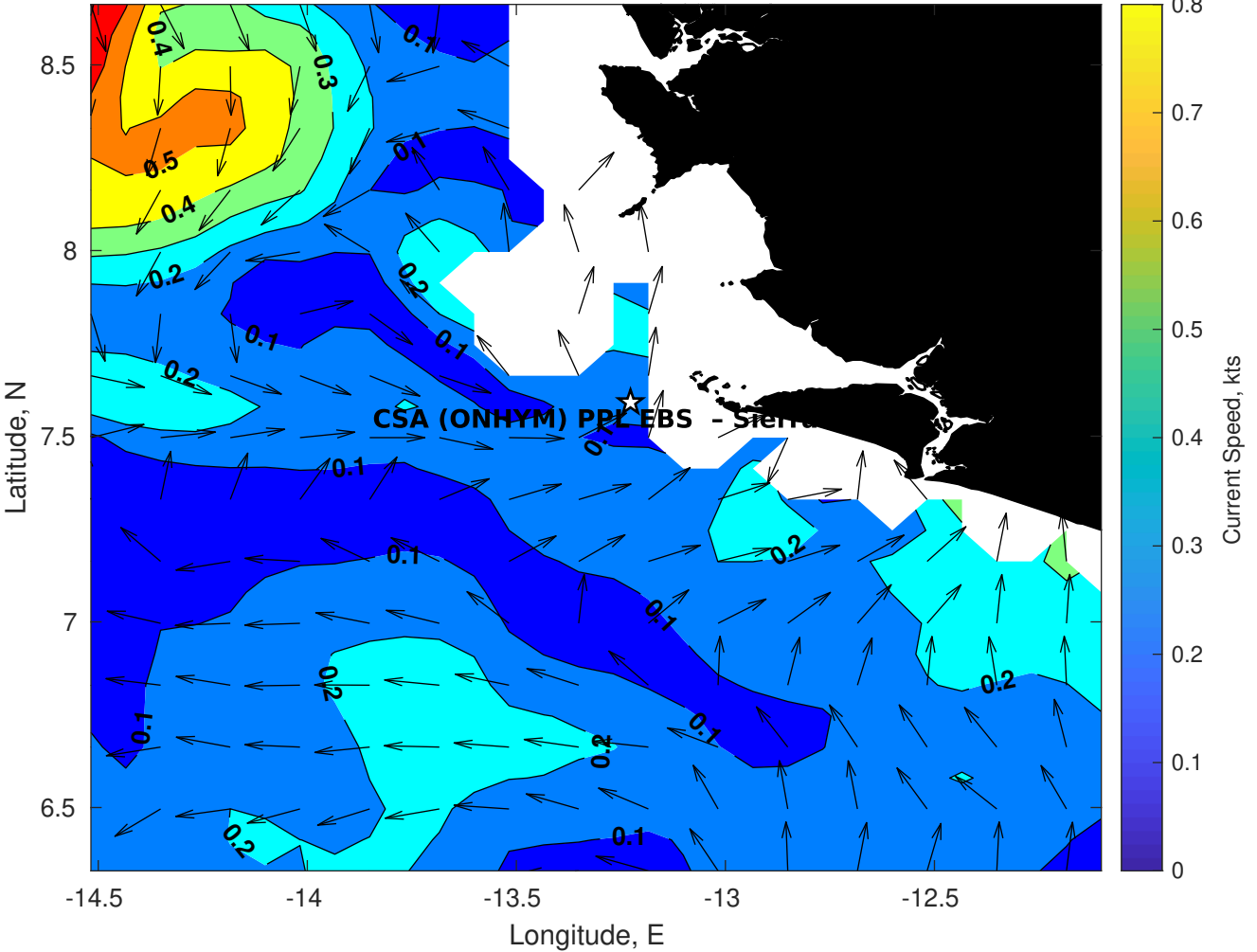
Surface Currents for CSA (ONHYM) PPL EBS - Sierra Leone at 21-Dec-2025 00:00:00
