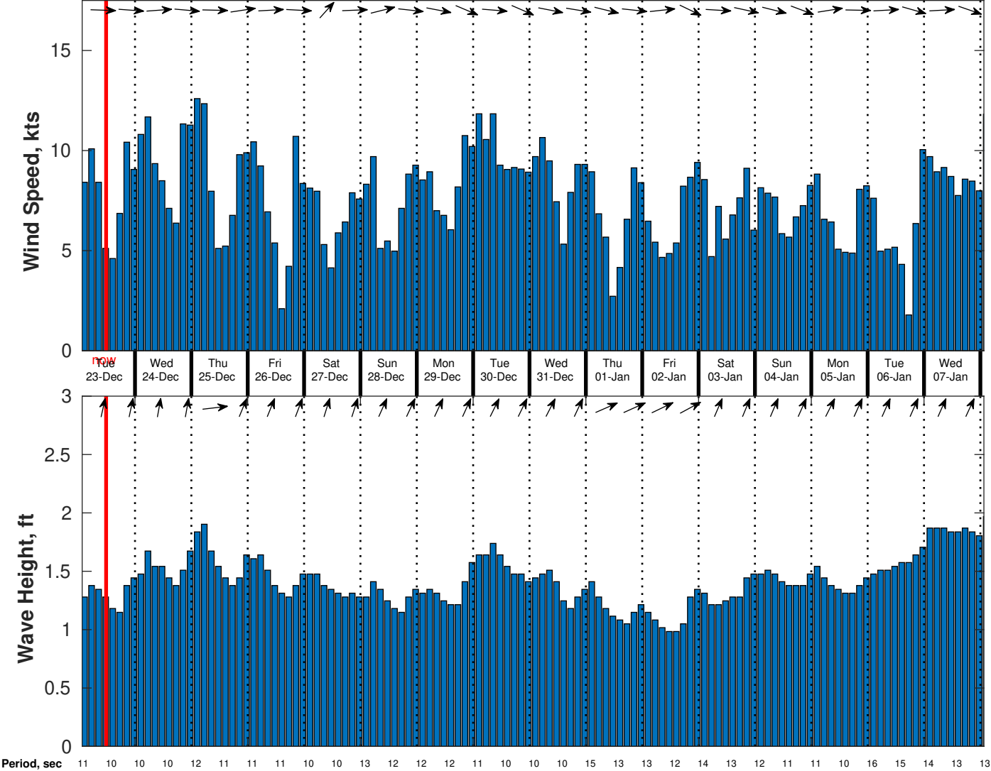
Wind & Wave Forecast for CSA (ONHYM) PPL EBS - Sierra Leone from 22-Dec-2025 01:00:00 to 07-Jan-2026 01:00:00
