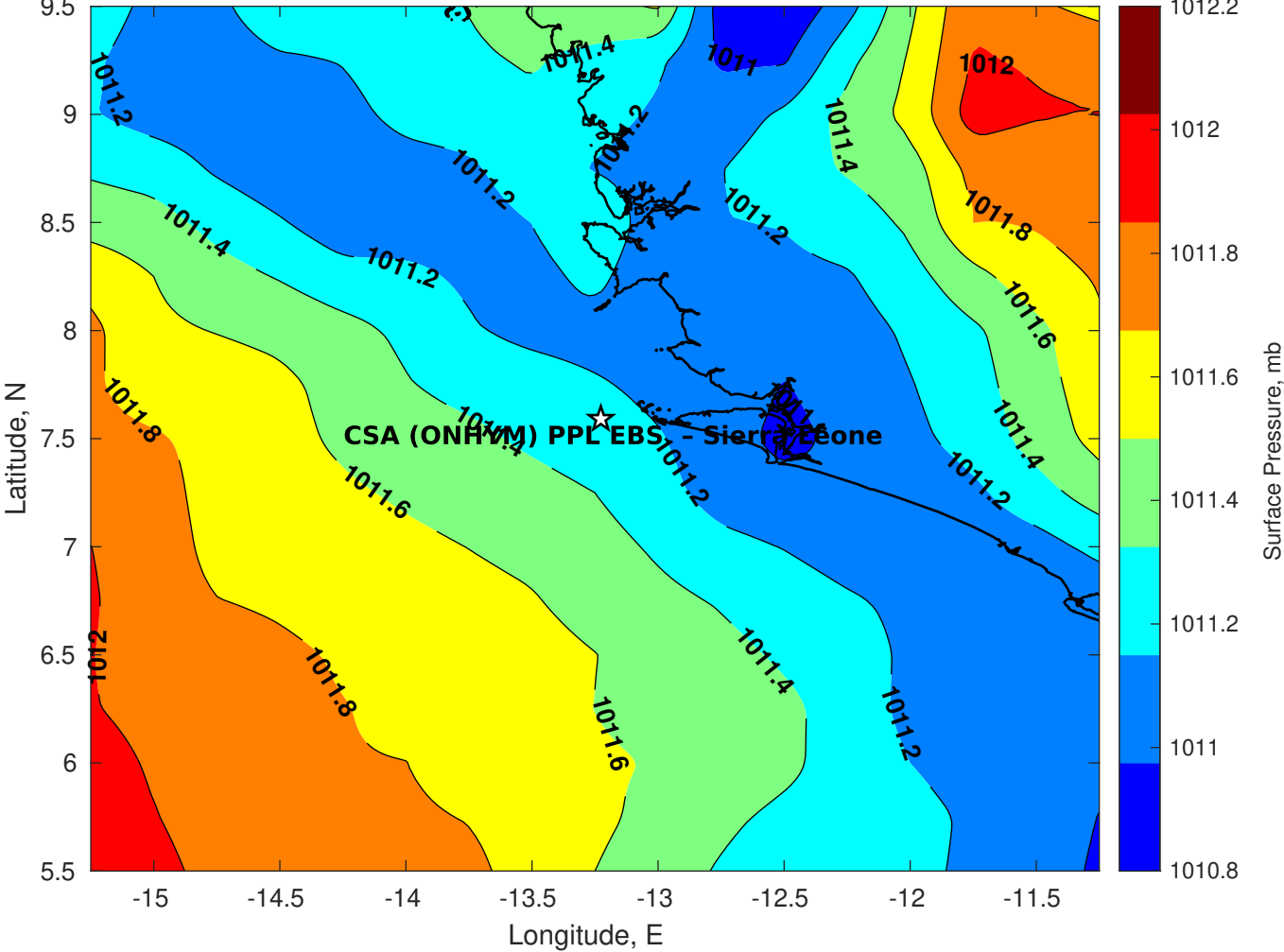
Surface Pressure (mb) for CSA (ONHYM) PPL EBS - Sierra Leone at 24-Dec-2025 00:00:00
