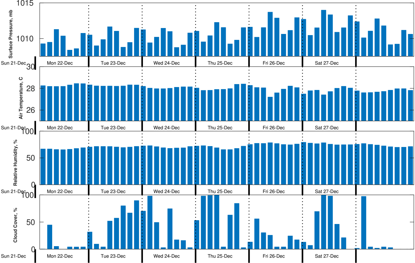
Met Forecast for CSA (ONHYM) PPL EBS - Sierra Leone from 22-Dec-2025 00:00:00 to 29-Dec-2025 00:00:00
