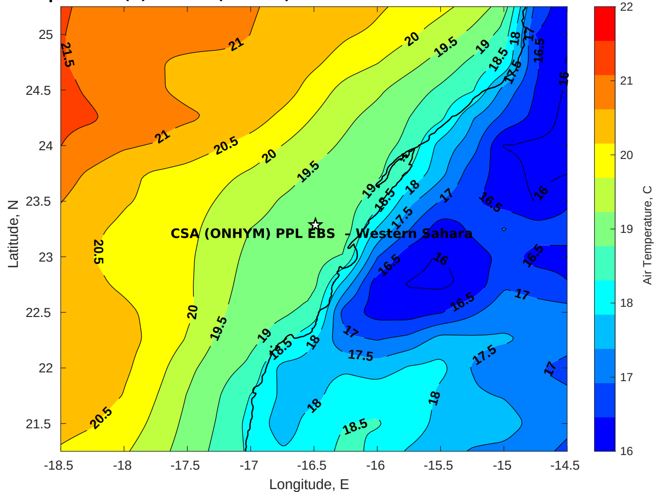
Air Temperature (C) for CSA (ONHYM) PPL EBS - Western Sahara at 22-Dec-2025
