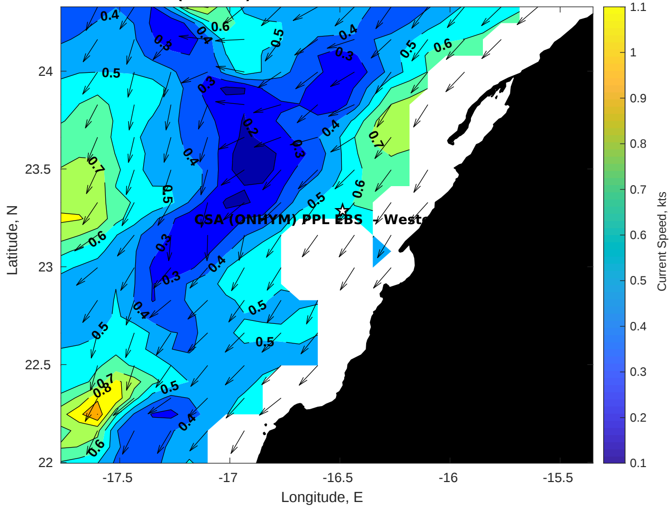
Surface Currents for CSA (ONHYM) PPL EBS - Western Sahara at 21-Dec-2025 00:00:00
