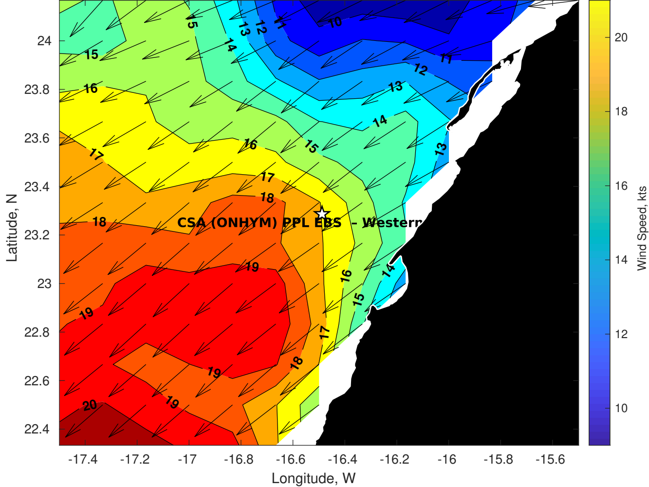
GFS Winds (kts) for CSA (ONHYM) PPL EBS - Western Sahara at 22-Dec-2025 09:00:00
