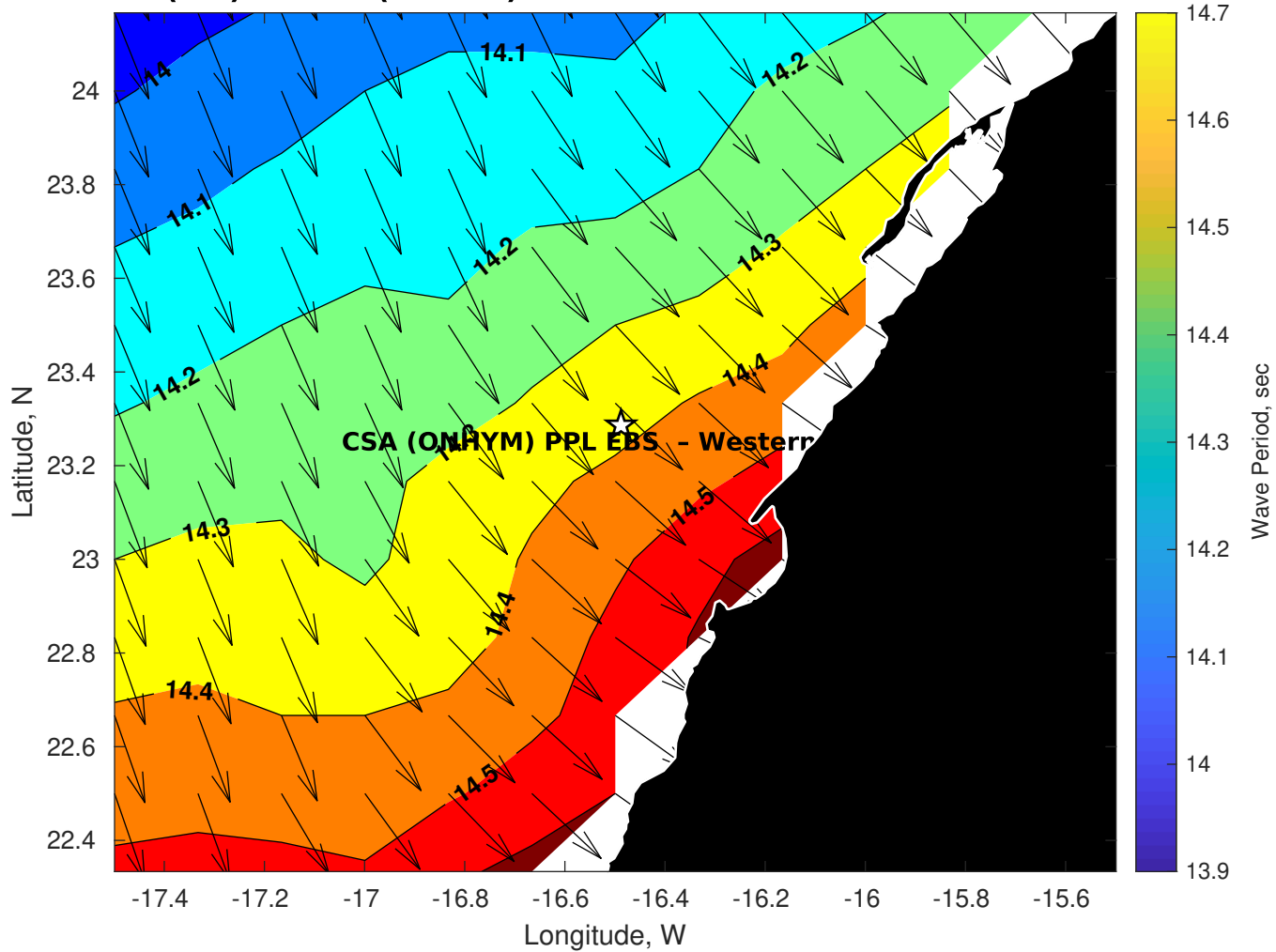
GFS Wave Period (sec) for CSA (ONHYM) PPL EBS - Western Sahara at 22-Dec-2025 09:00:00
