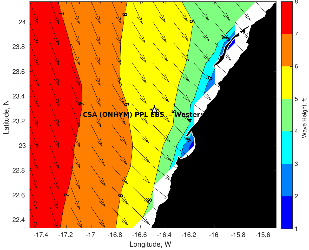
GFS Wave Height (ft) for CSA (ONHYM) PPL EBS - Western Sahara at 22-Dec-2025 09:00:00
