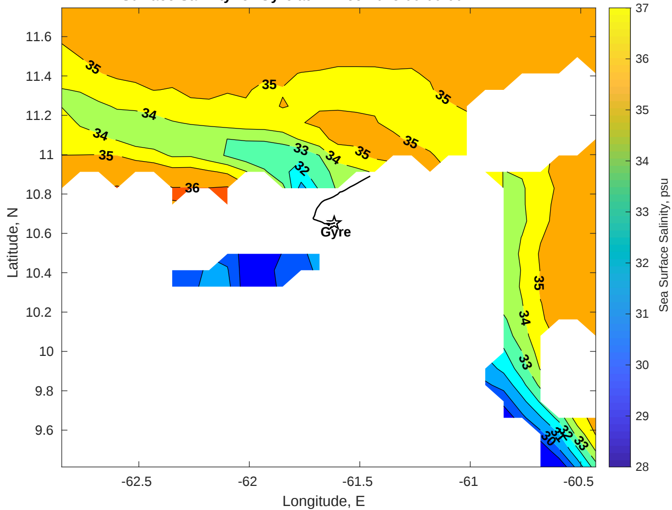
Surface Salinity for Gyre at 21-Dec-2025 00:00:00
