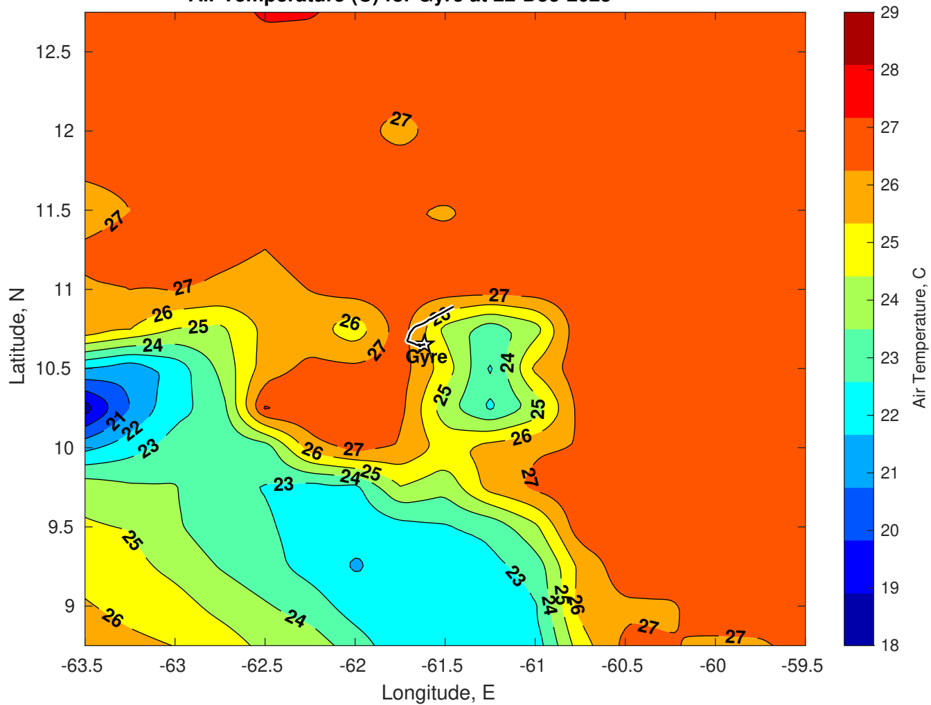
Air Temperature (C) for Gyre at 22-Dec-2025
