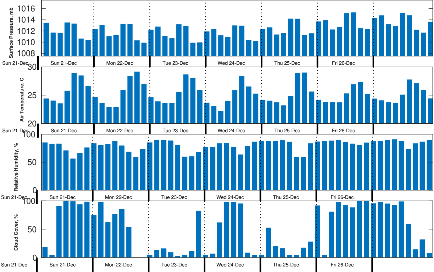
Met Forecast for Gyre from 21-Dec-2025 20:00:00 to 28-Dec-2025 20:00:00
