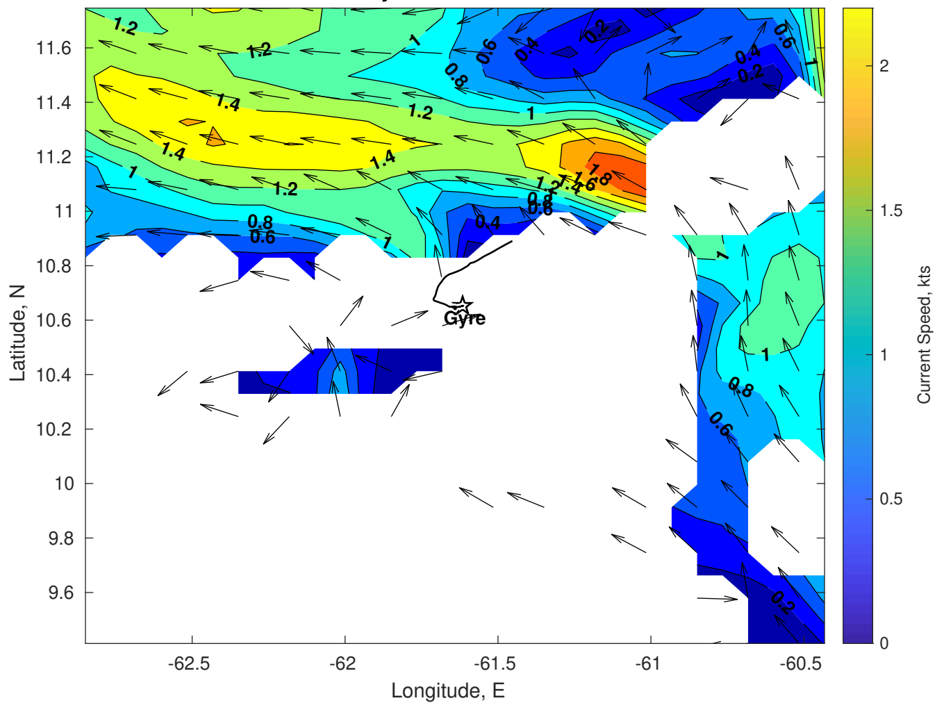
Surface Currents for Gyre at 21-Dec-2025 00:00:00
