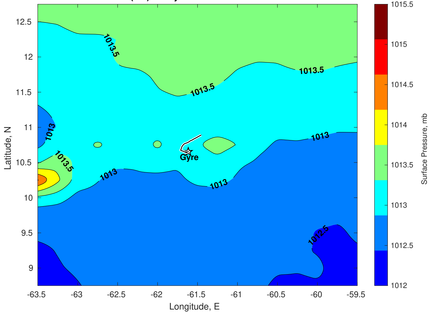
Surface Pressure (mb) for Gyre at 22-Dec-2025 00:00:00
