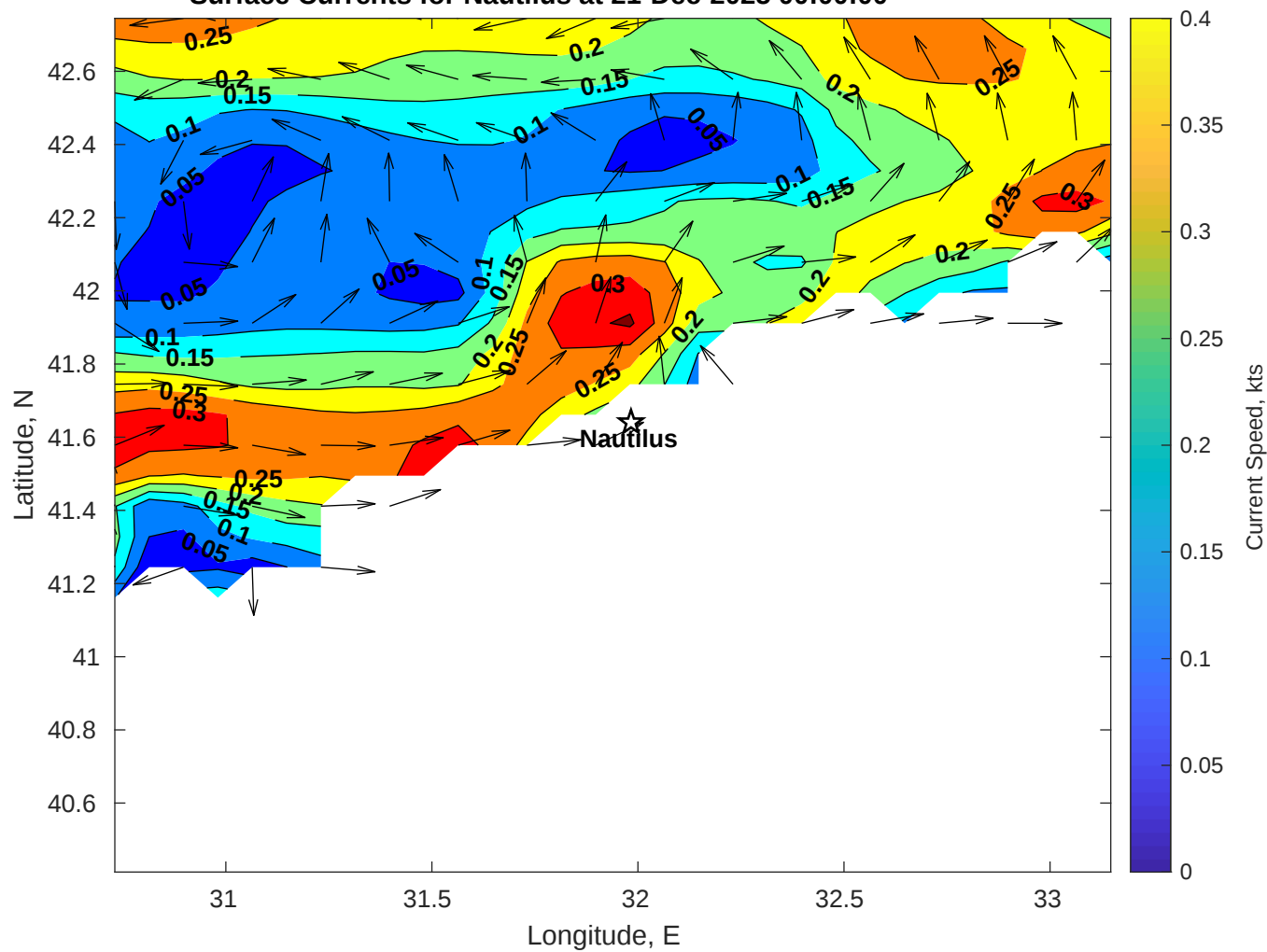
Surface Currents for Nautilus at 21-Dec-2025 00:00:00
