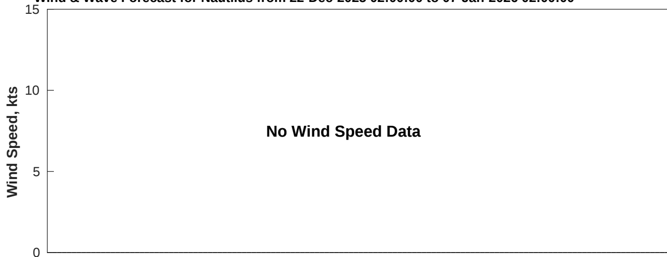
Wind & Wave Forecast for Nautilus from 22-Dec-2025 02:00:00 to 07-Jan-2026 02:00:00
