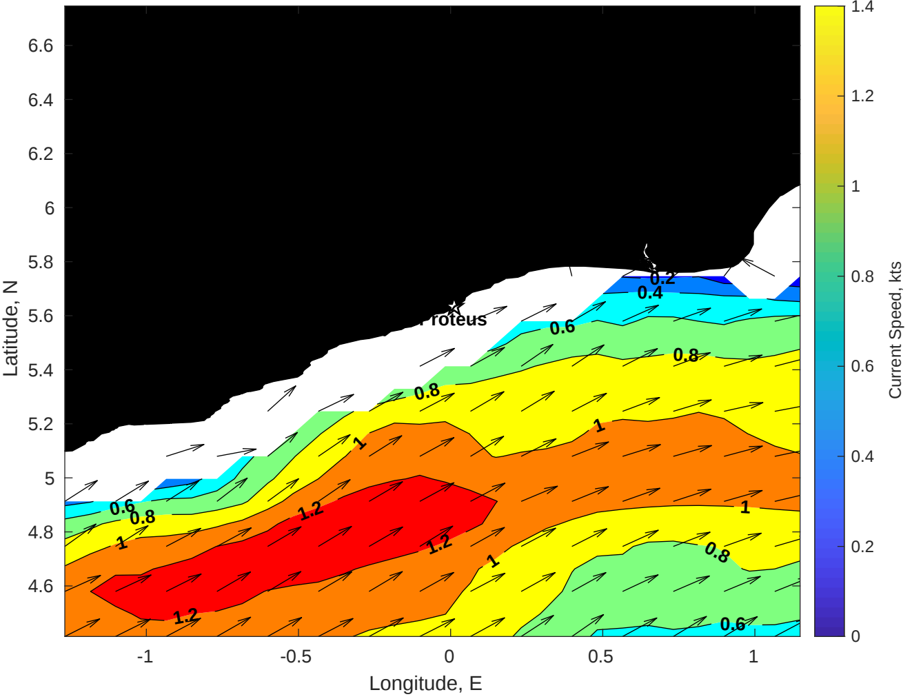
Surface Currents for Proteus at 21-Dec-2025 00:00:00
