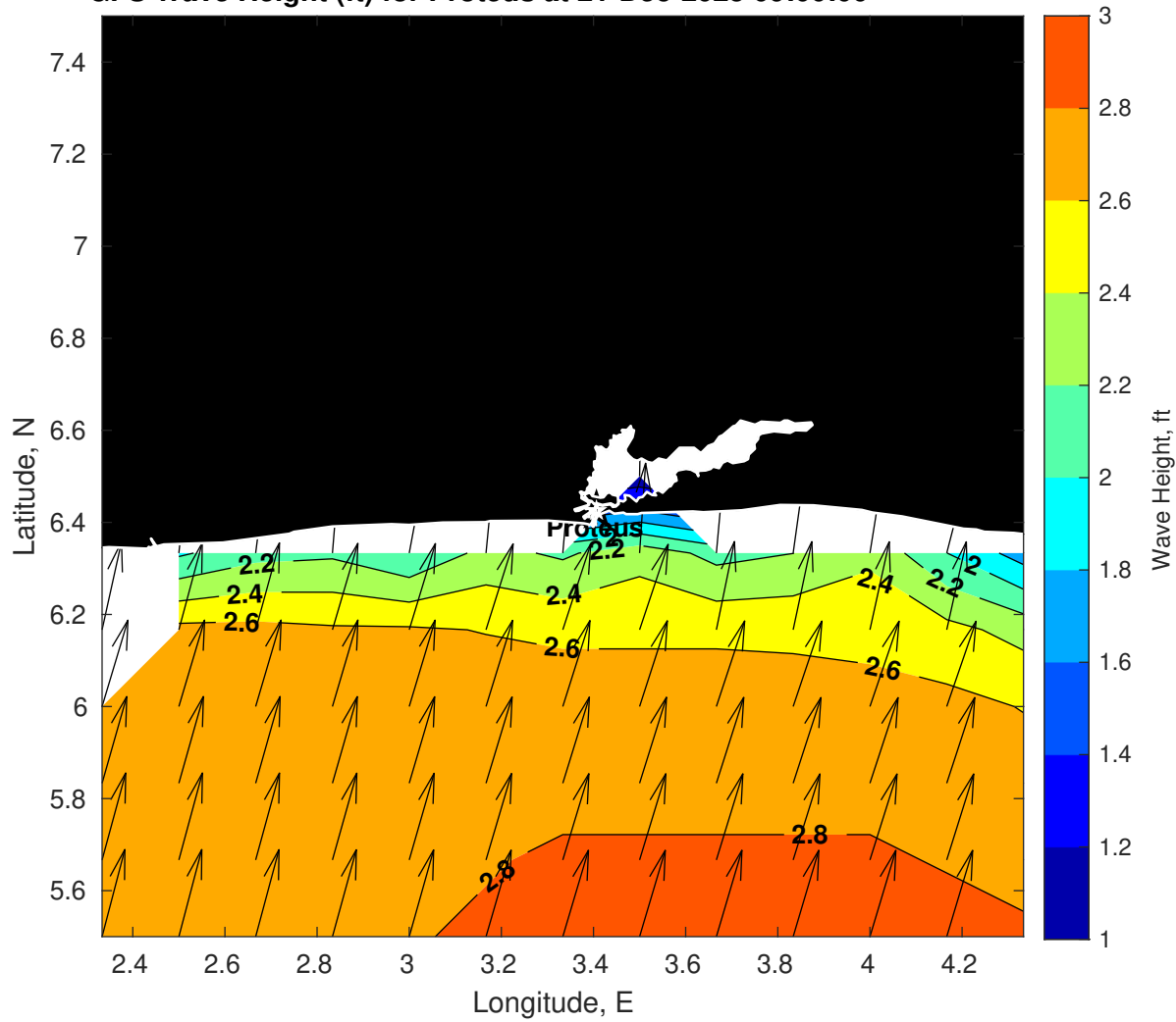
GFS Wave Height (ft) for Proteus at 21-Dec-2025 09:00:00
