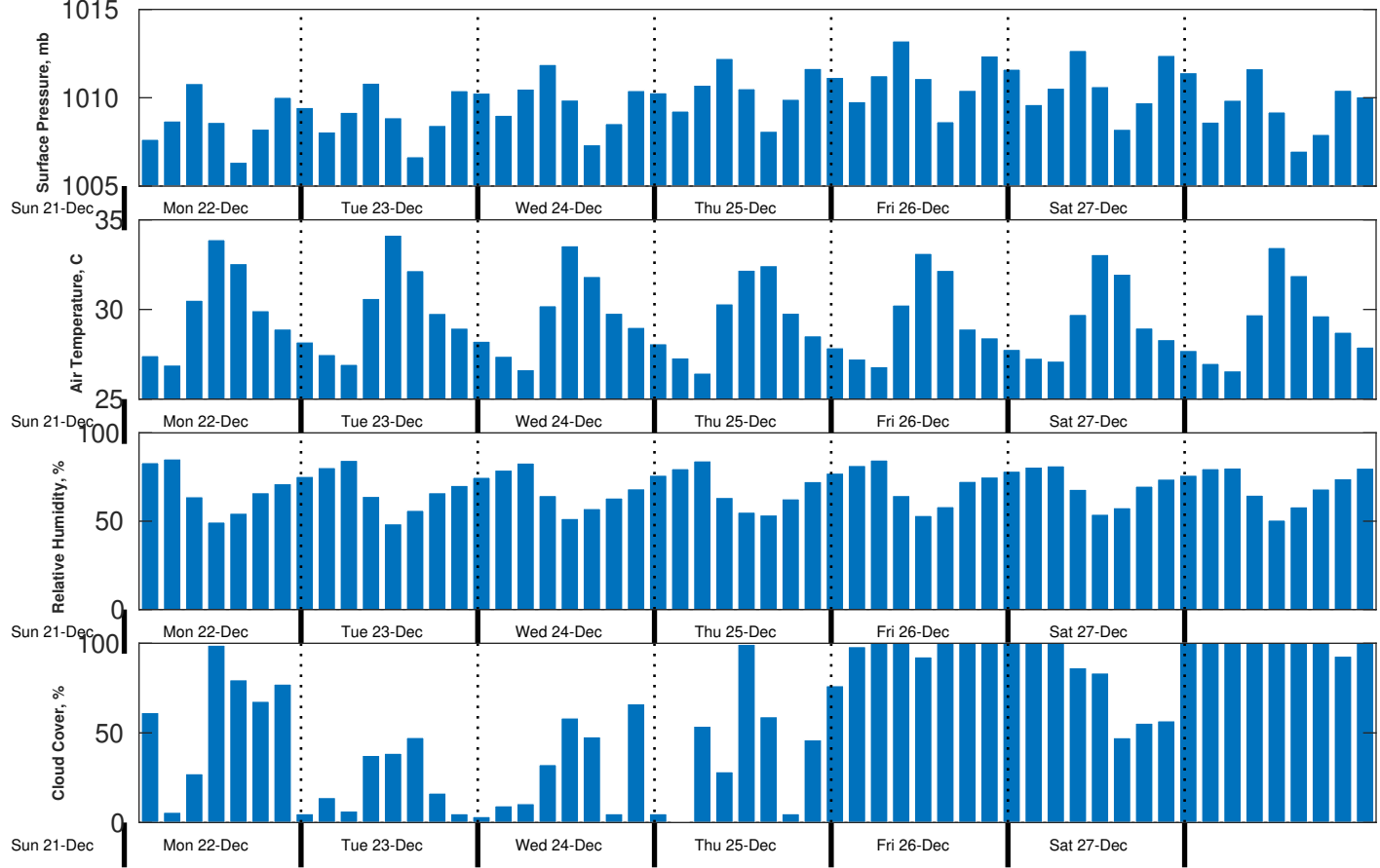
Met Forecast for Proteus from 22-Dec-2025 00:00:00 to 29-Dec-2025 00:00:00
