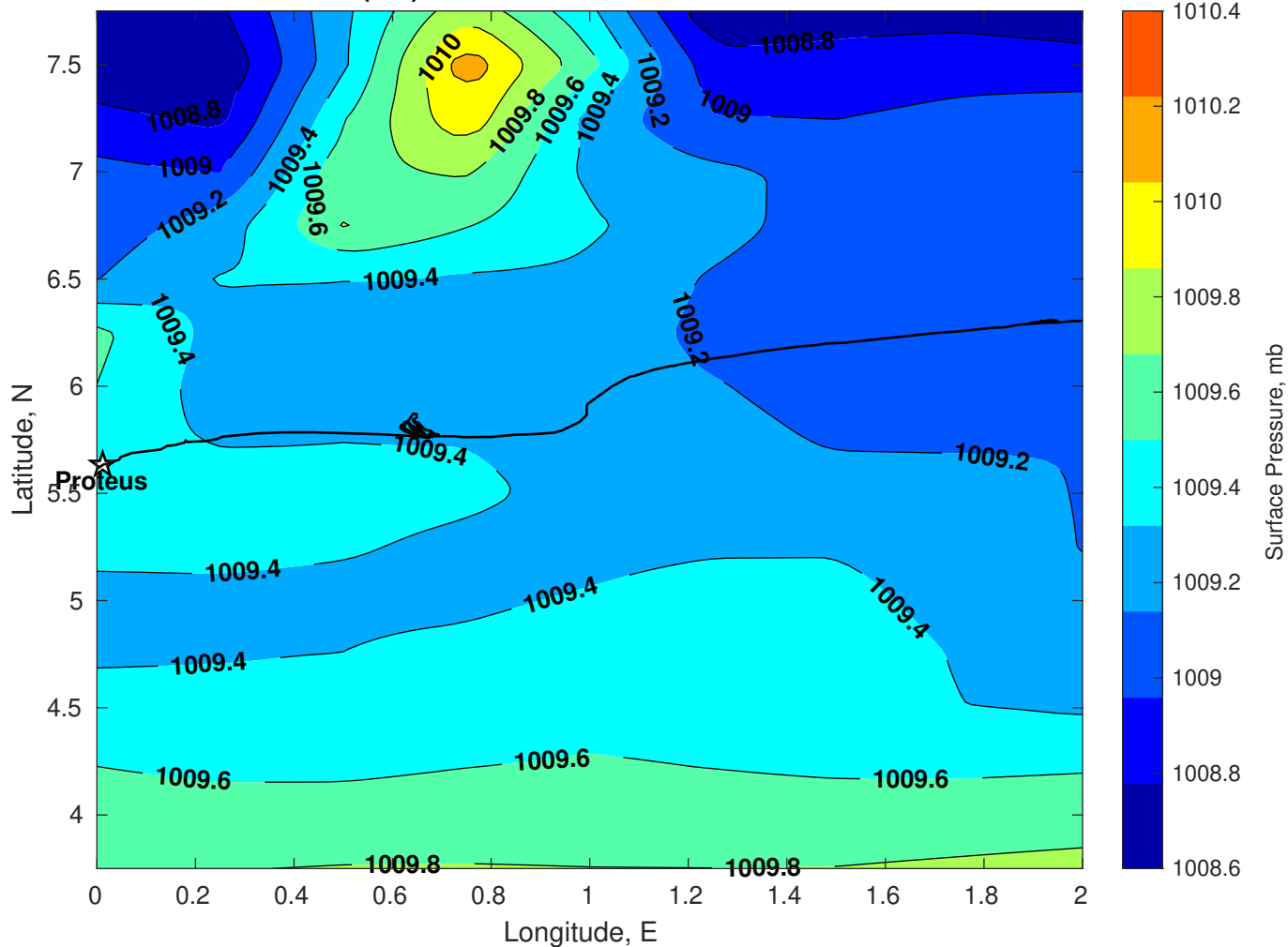
Surface Pressure (mb) for Proteus at 23-Dec-2025 00:00:00
