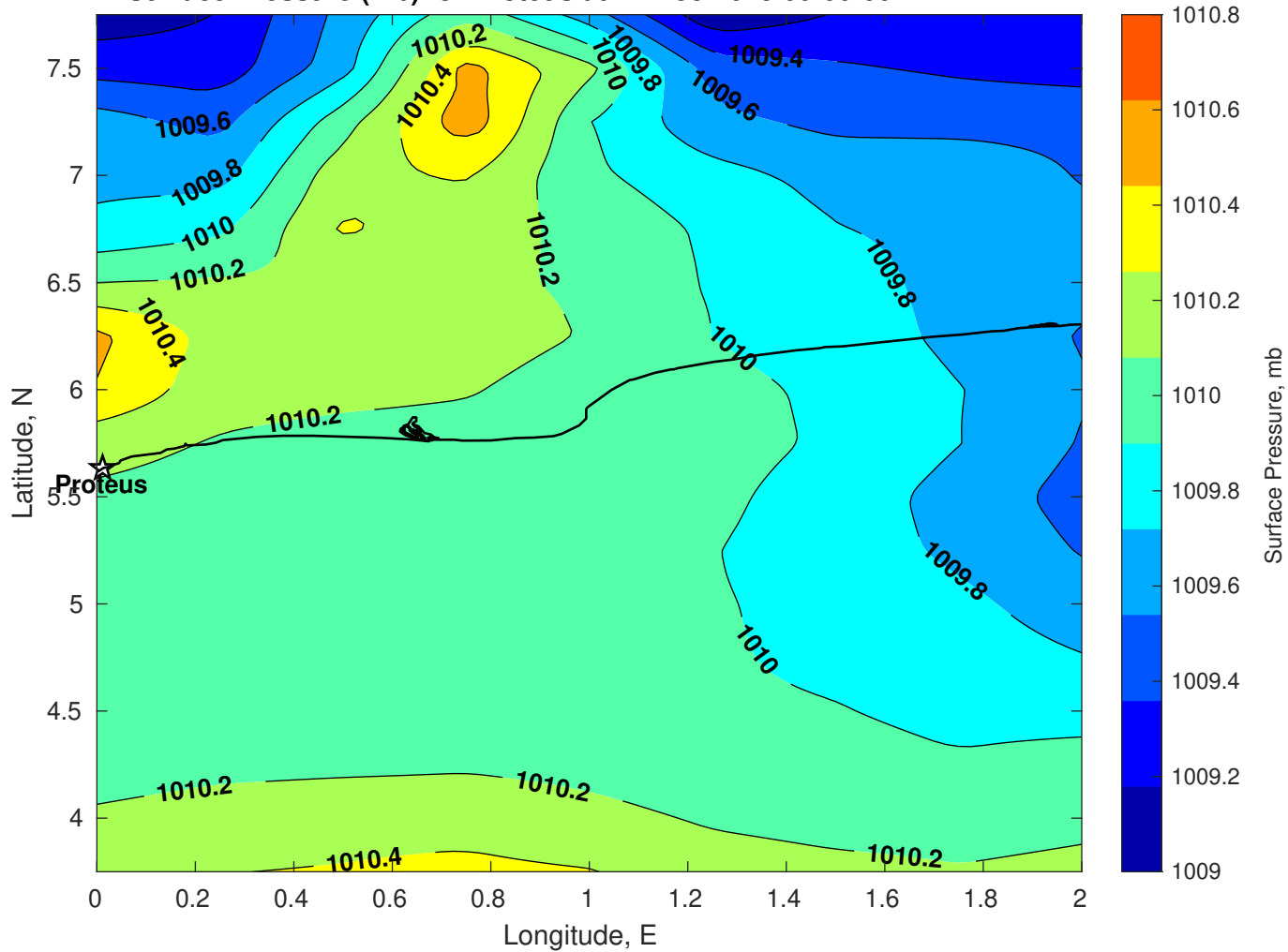
Surface Pressure (mb) for Proteus at 24-Dec-2025 00:00:00
