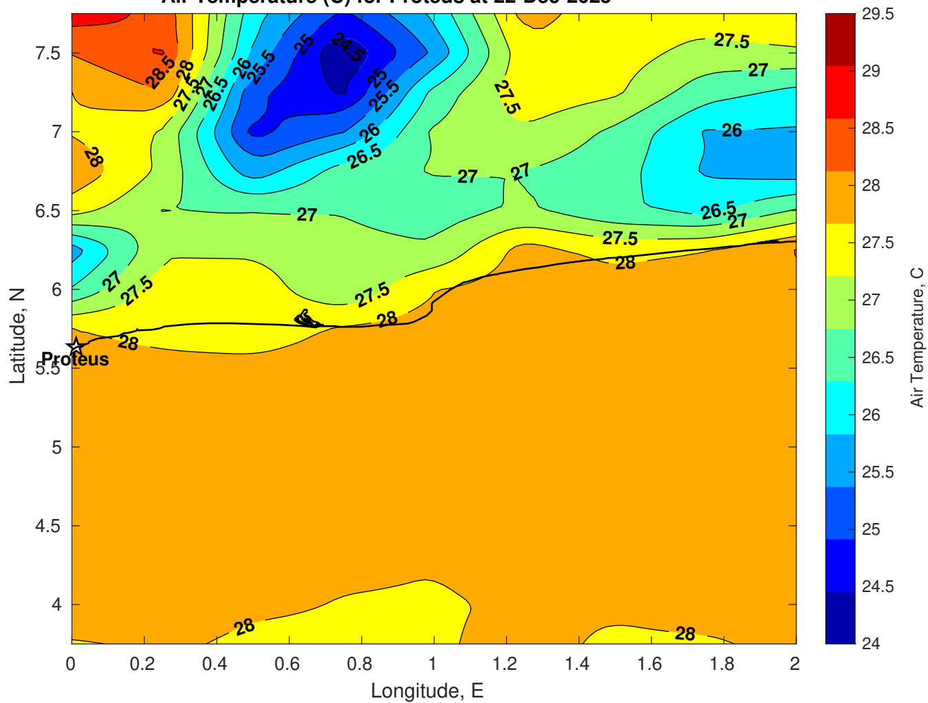
Air Temperature (C) for Proteus at 22-Dec-2025
