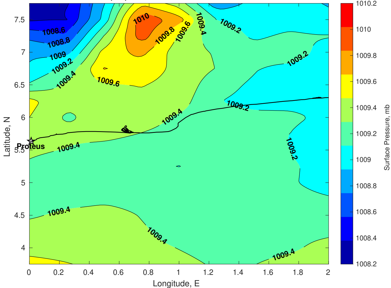
Surface Pressure (mb) for Proteus at 22-Dec-2025 00:00:00
