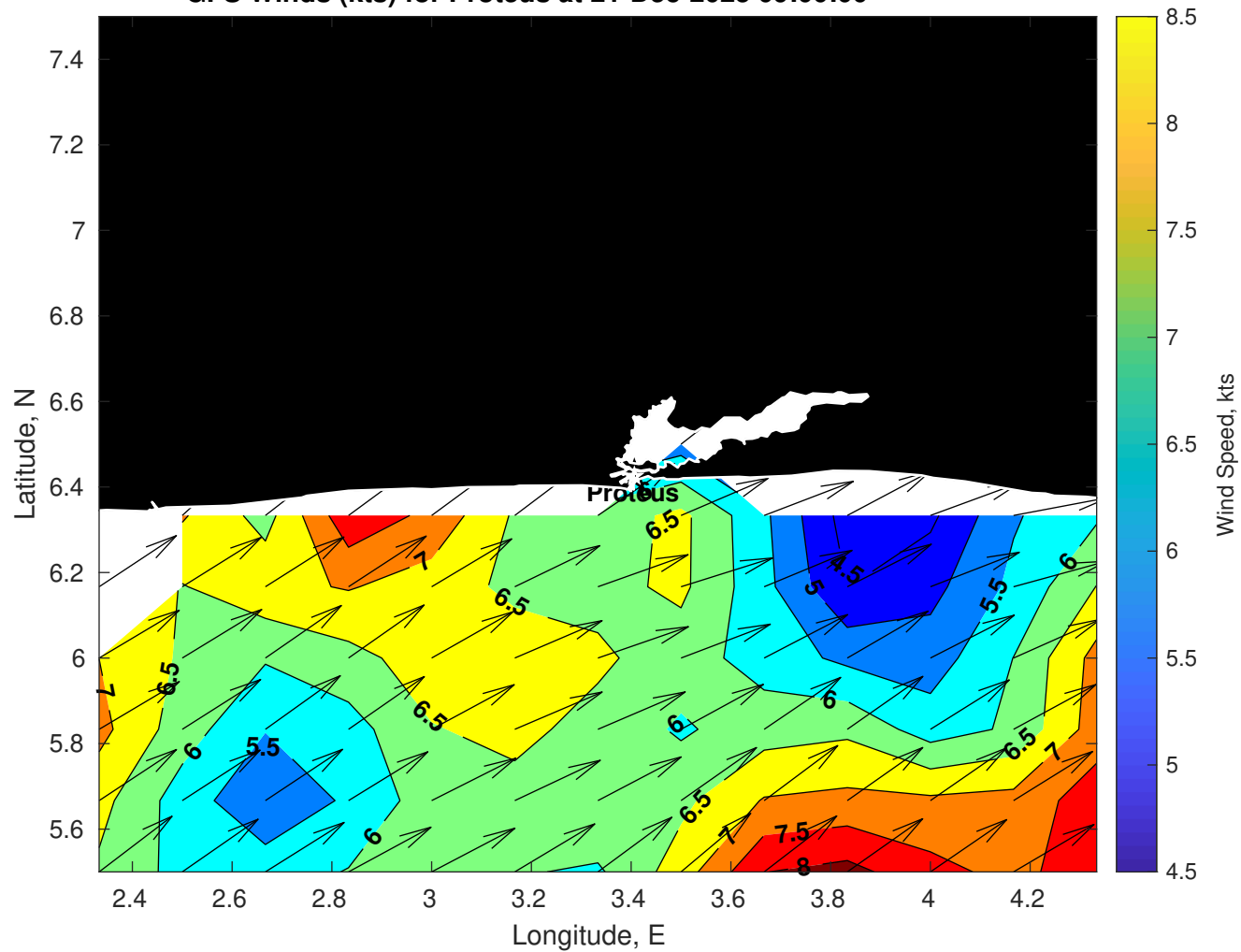
GFS Winds (kts) for Proteus at 21-Dec-2025 09:00:00
