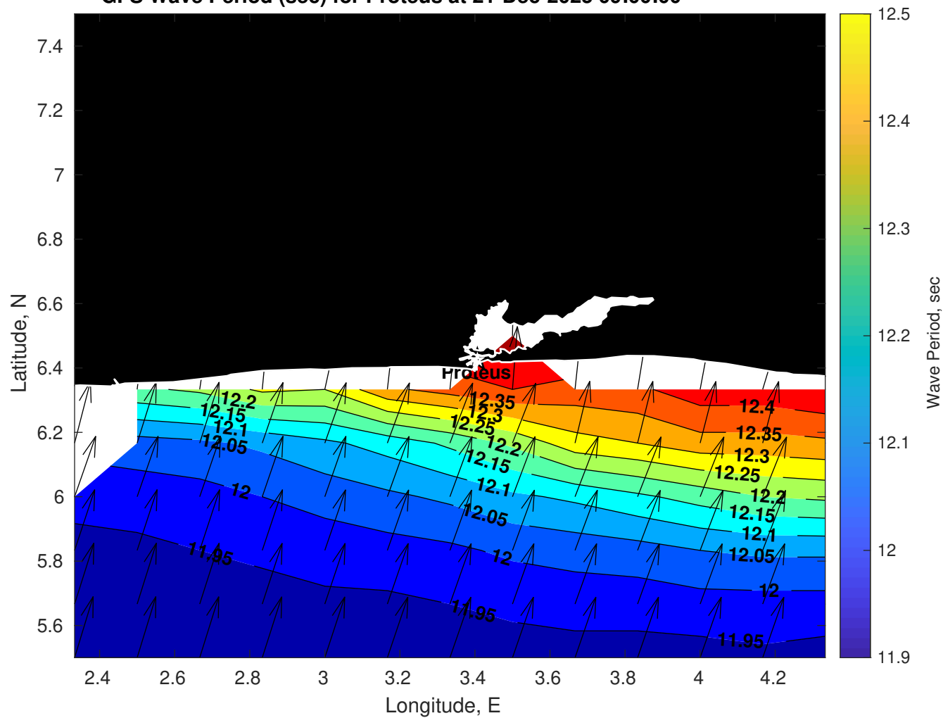
GFS Wave Period (sec) for Proteus at 21-Dec-2025 09:00:00
