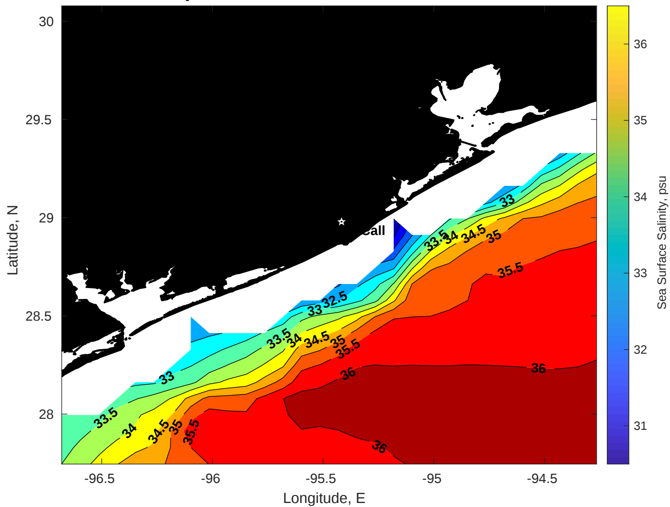
Surface Salinity for Brooks McCall at 22-Dec-2025 00:00:00
