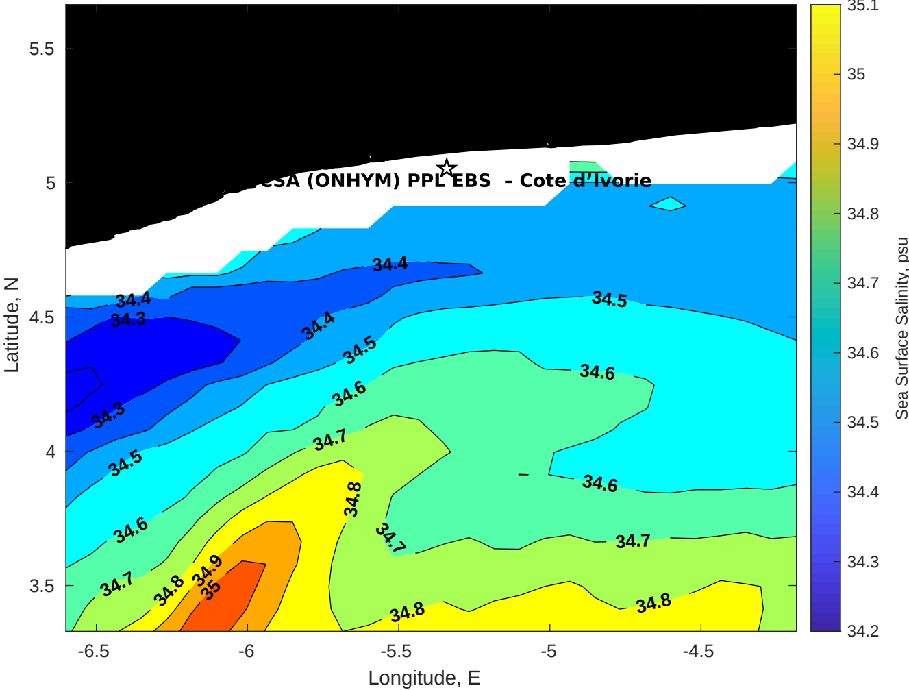
Surface Salinity for CSA (ONHYM) PPL EBS - Cote d'Ivoire at 22-Dec-2025 00:00:00
