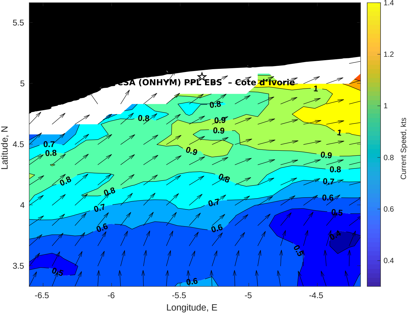
Surface Currents for CSA (ONHYM) PPL EBS - Cote d'Ivoire at 22-Dec-2025 00:00:00
