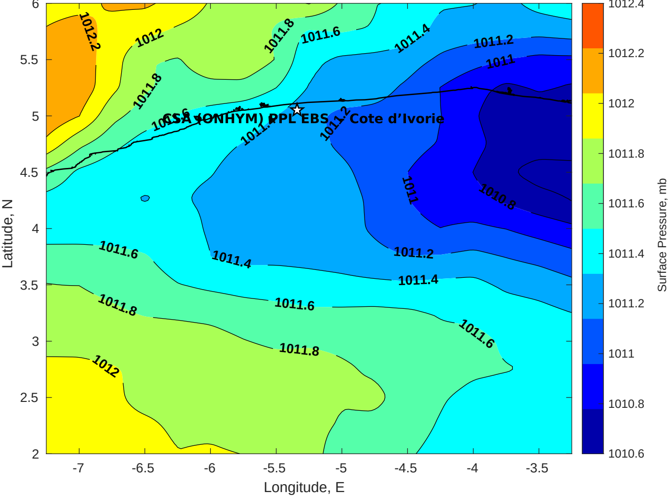
Surface Pressure (mb) for CSA (ONHYM) PPL EBS - Cote d'Ivoire at 24-Dec-2025 00:00:00
