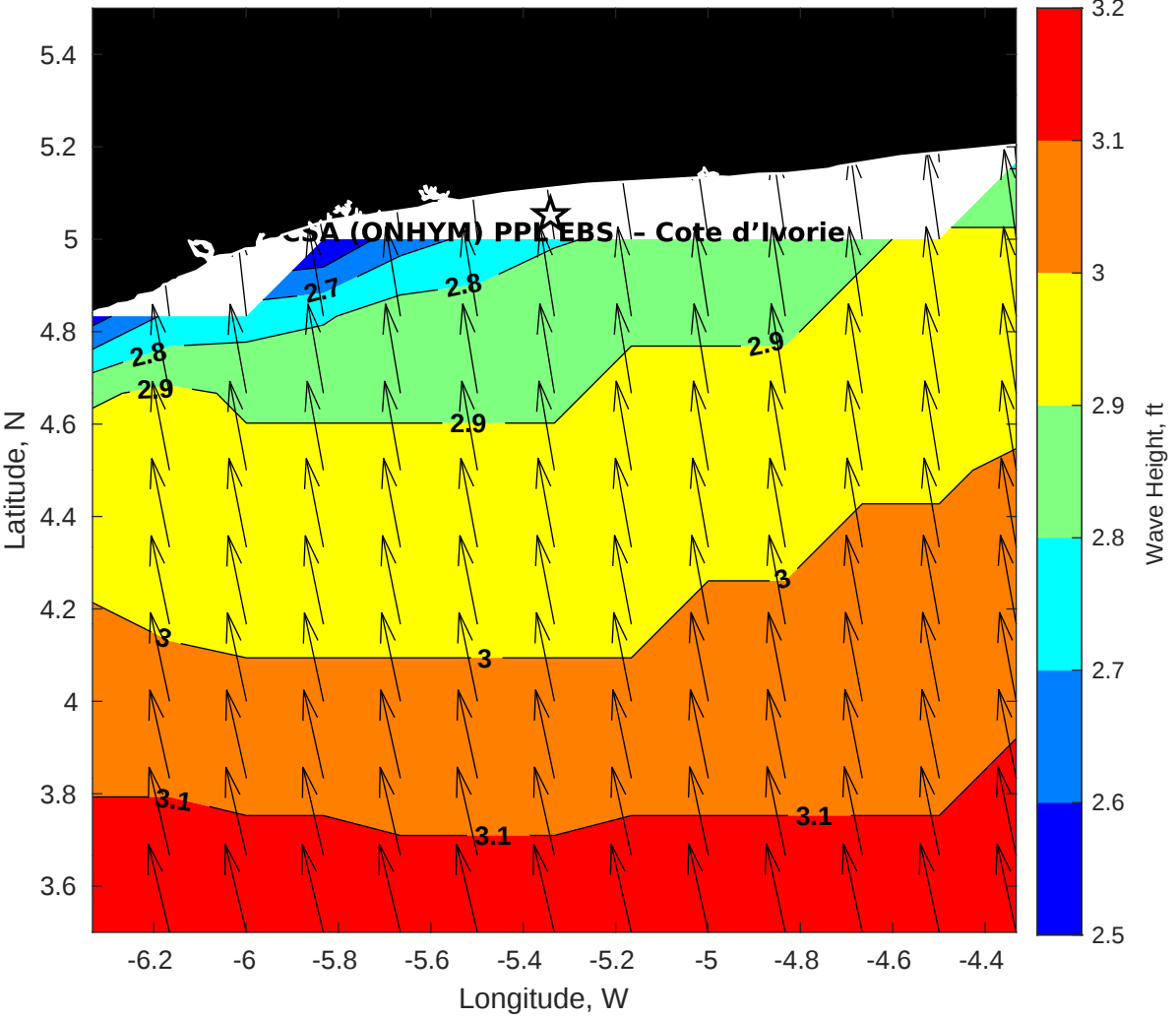
GFS Wave Height (ft) for CSA (ONHYM) PPL EBS - Cote d'Ivoire at 23-Dec-2025 09:00:00
