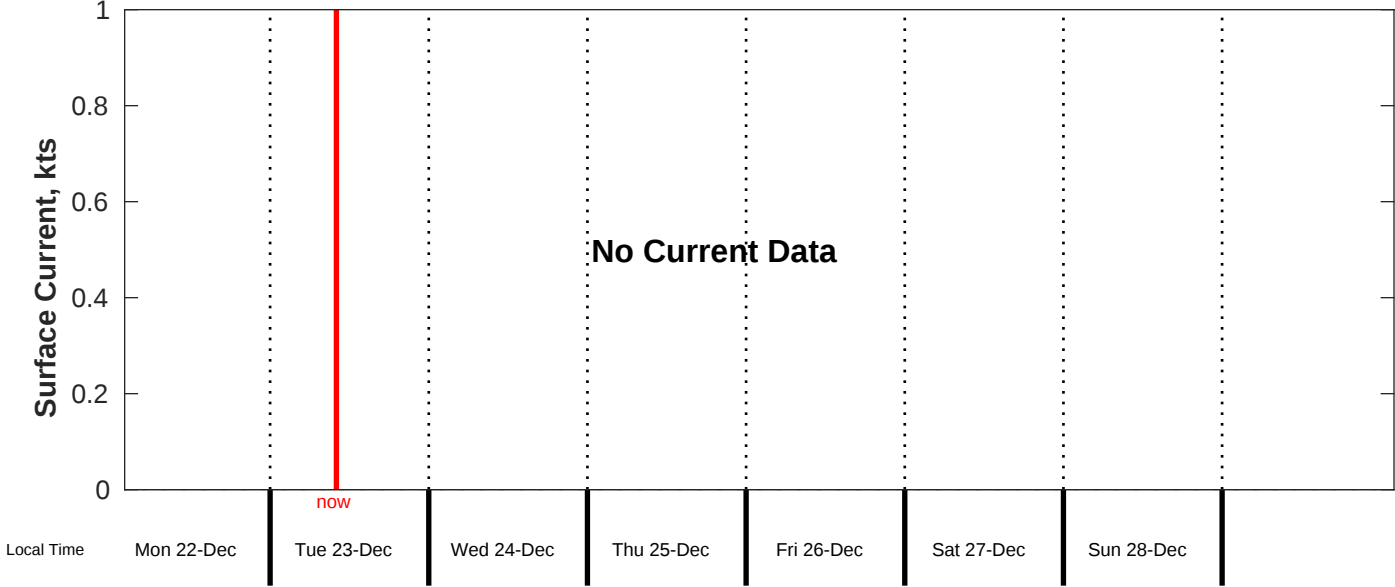
Surface Current Forecast for CSA (ONHYM) PPL EBS - Cote d'Ivoire from 22-Dec-2025 00:00:00 to 30-Dec-2025 00:00:00
