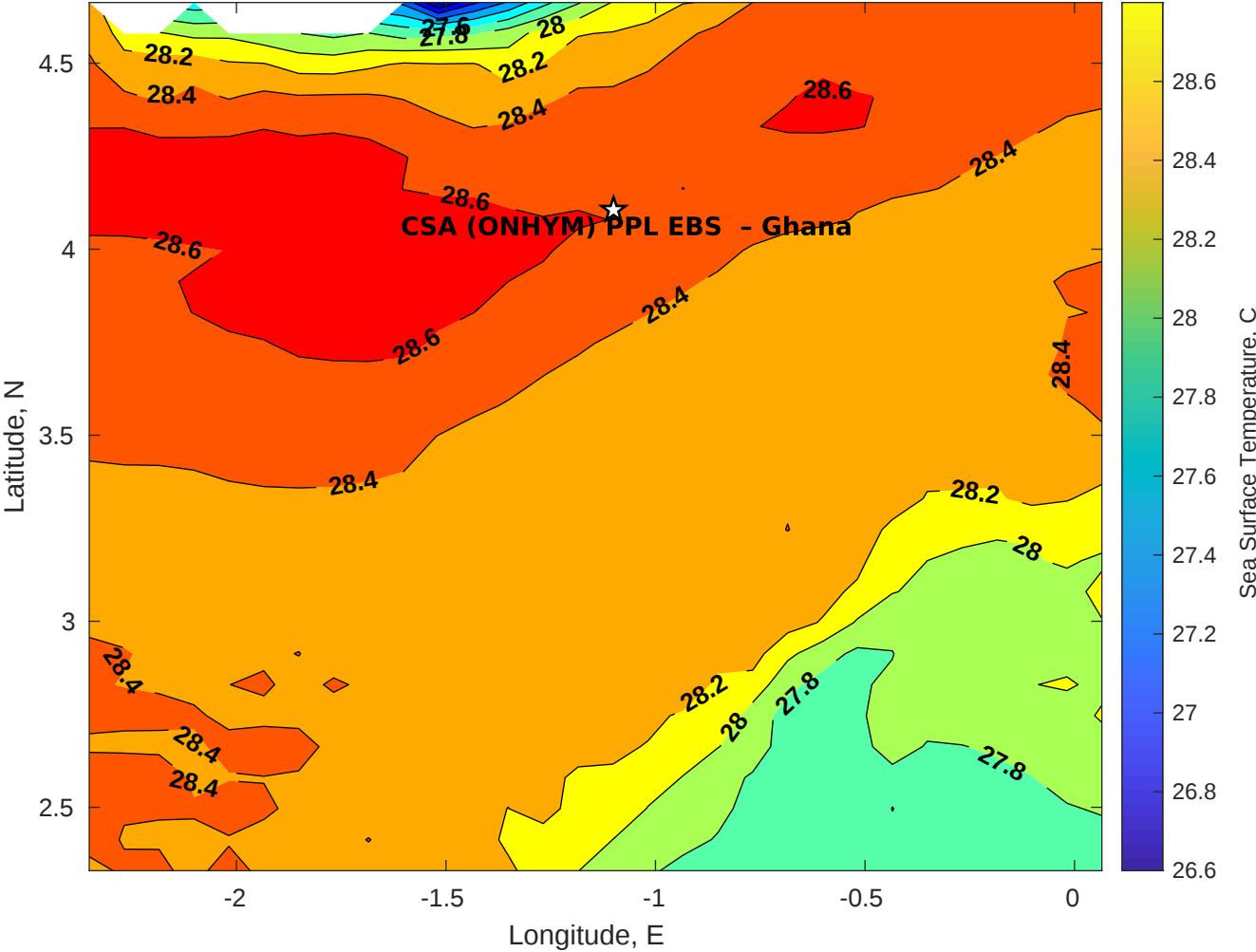
SST for CSA (ONHYM) PPL EBS - Ghana at 22-Dec-2025 00:00:00
