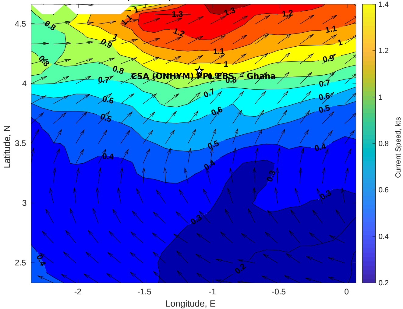
Surface Currents for CSA (ONHYM) PPL EBS - Ghana at 22-Dec-2025 00:00:00
