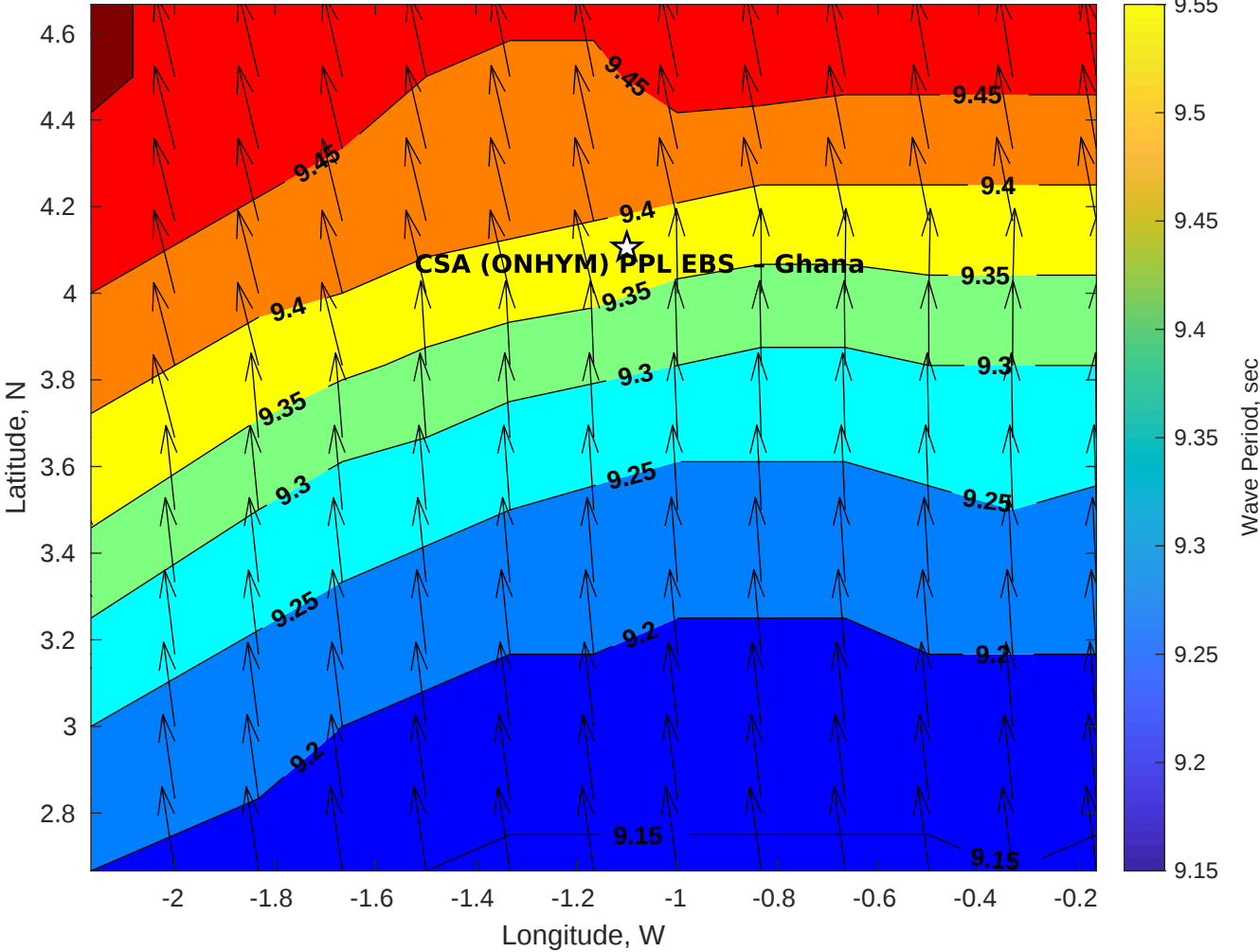
GFS Wave Period (sec) for CSA (ONHYM) PPL EBS - Ghana at 23-Dec-2025 09:00:00
